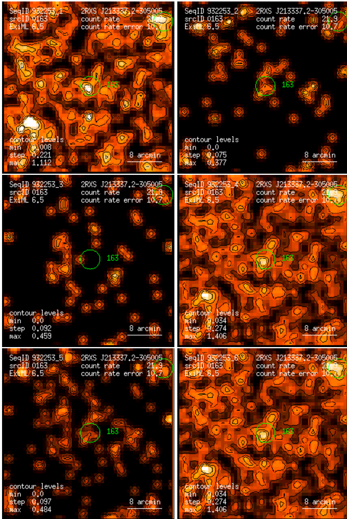
Figure 163: RASS 932253: detection 0163: band rate images, Gaussian filter: (1) PSPC channels 11 – 41, (2) 52 – 90, (3) 91 – 201, (4) 11 – 235, (5) 52 – 201, (6) 11 – 201. Broad band rates in counts/ks. Band rate contour levels in counts/ks/arcmin 2 .
