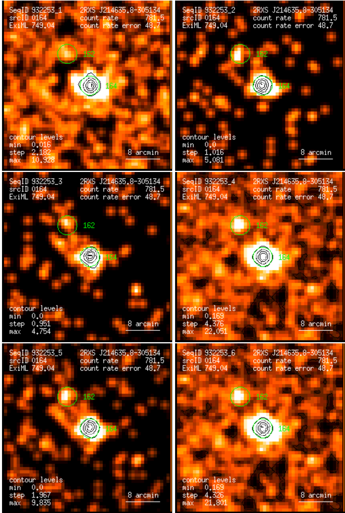
Figure 164: RASS 932253: detection 0164: band rate images, Gaussian filter: (1) PSPC channels 11 – 41, (2) 52 – 90, (3) 91 – 201, (4) 11 – 235, (5) 52 – 201, (6) 11 – 201. Broad band rates in counts/ks. Band rate contour levels in counts/ks/arcmin 2 .
