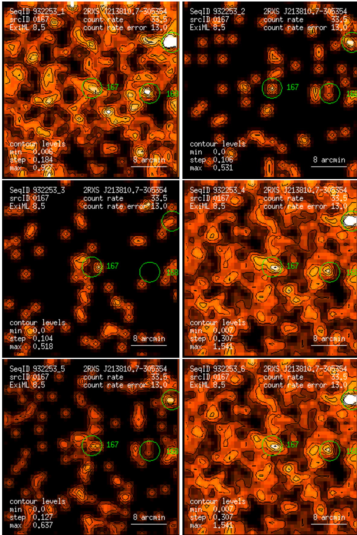
Figure 167: RASS 932253: detection 0167: band rate images, Gaussian filter: (1) PSPC channels 11 – 41, (2) 52 – 90, (3) 91 – 201, (4) 11 – 235, (5) 52 – 201, (6) 11 – 201. Broad band rates in counts/ks. Band rate contour levels in counts/ks/arcmin 2 .
