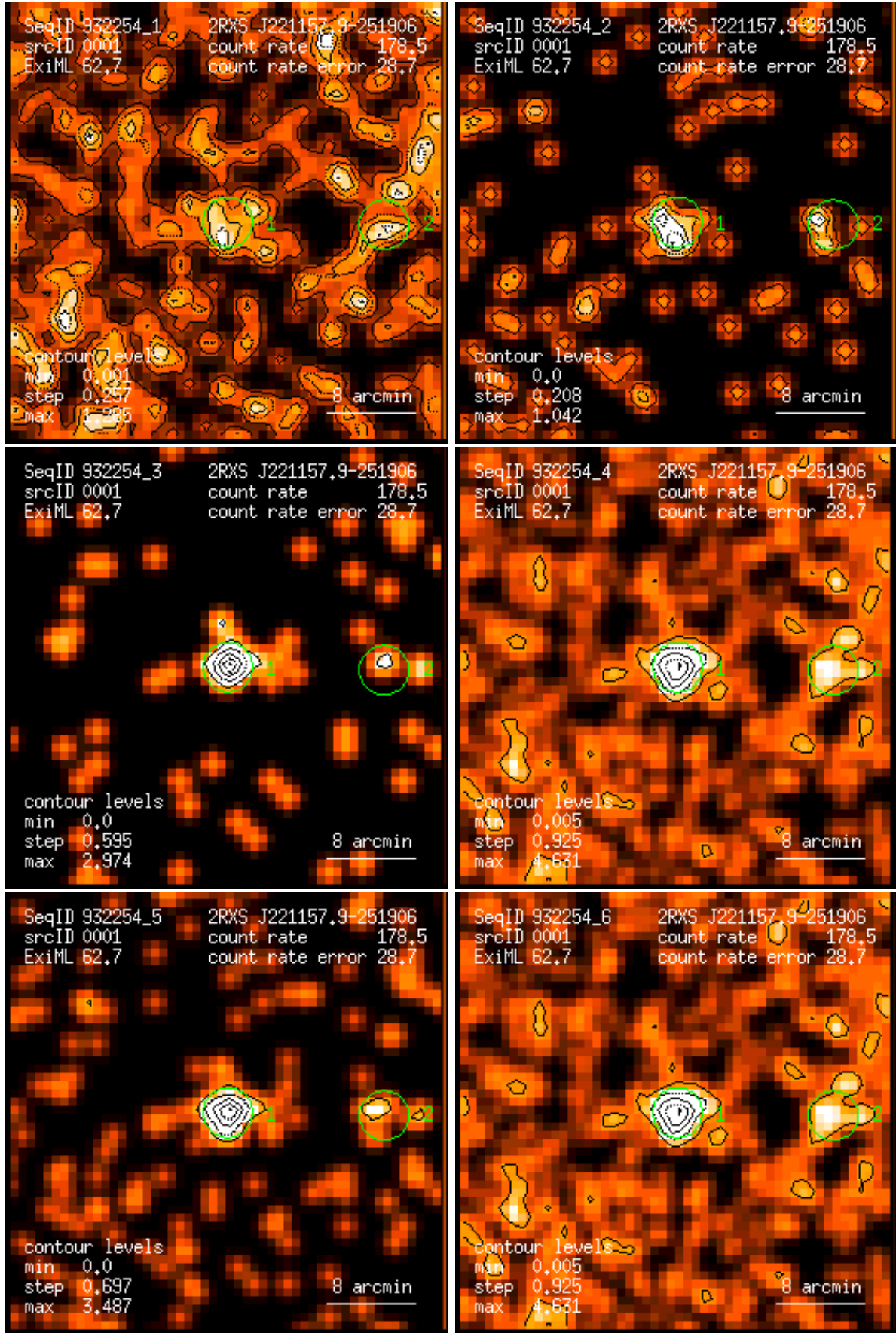
Figure 1: RASS 932254: detection 0001: band rate images, Gaussian filter: (1) PSPC channels 11 – 41, (2) 52 – 90, (3) 91 – 201, (4) 11 – 235, (5) 52 – 201, (6) 11 – 201. Broad band rates in counts/ks. Band rate contour levels in counts/ks/arcmin 2 .
