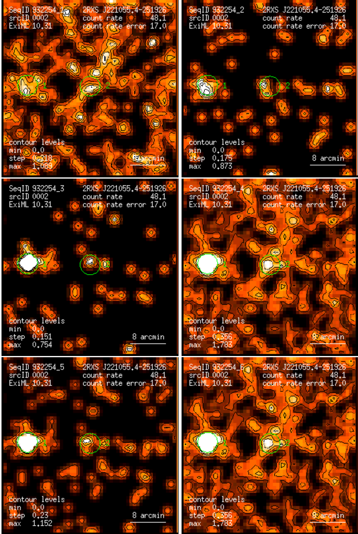
Figure 2: RASS 932254: detection 0002: band rate images, Gaussian filter: (1) PSPC channels 11 – 41, (2) 52 – 90, (3) 91 – 201, (4) 11 – 235, (5) 52 – 201, (6) 11 – 201. Broad band rates in counts/ks. Band rate contour levels in counts/ks/arcmin 2 .
