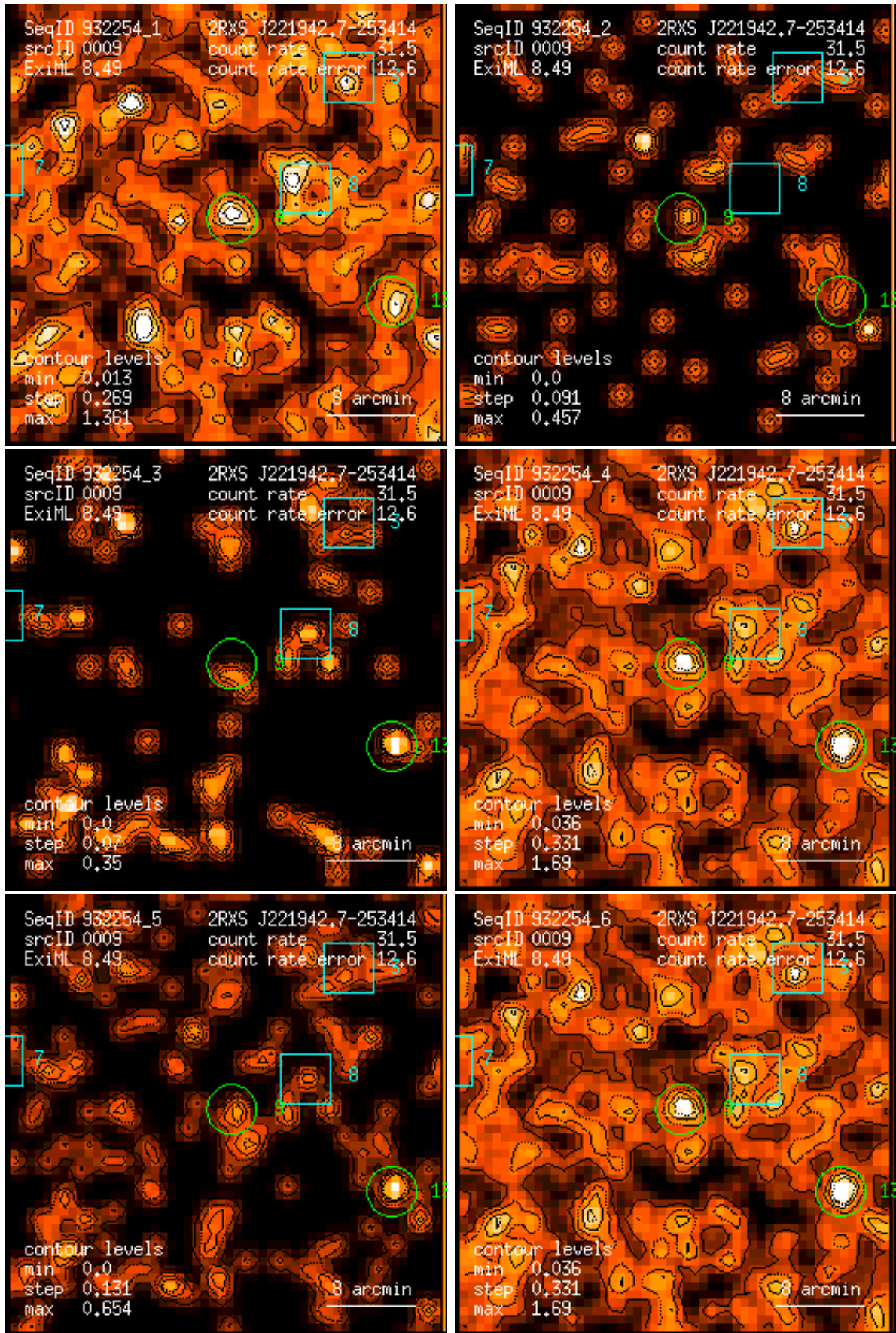
Figure 9: RASS 932254: detection 0009: band rate images, Gaussian filter: (1) PSPC channels 11 – 41, (2) 52 – 90, (3) 91 – 201, (4) 11 – 235, (5) 52 – 201, (6) 11 – 201. Broad band rates in counts/ks. Band rate contour levels in counts/ks/arcmin 2 .
