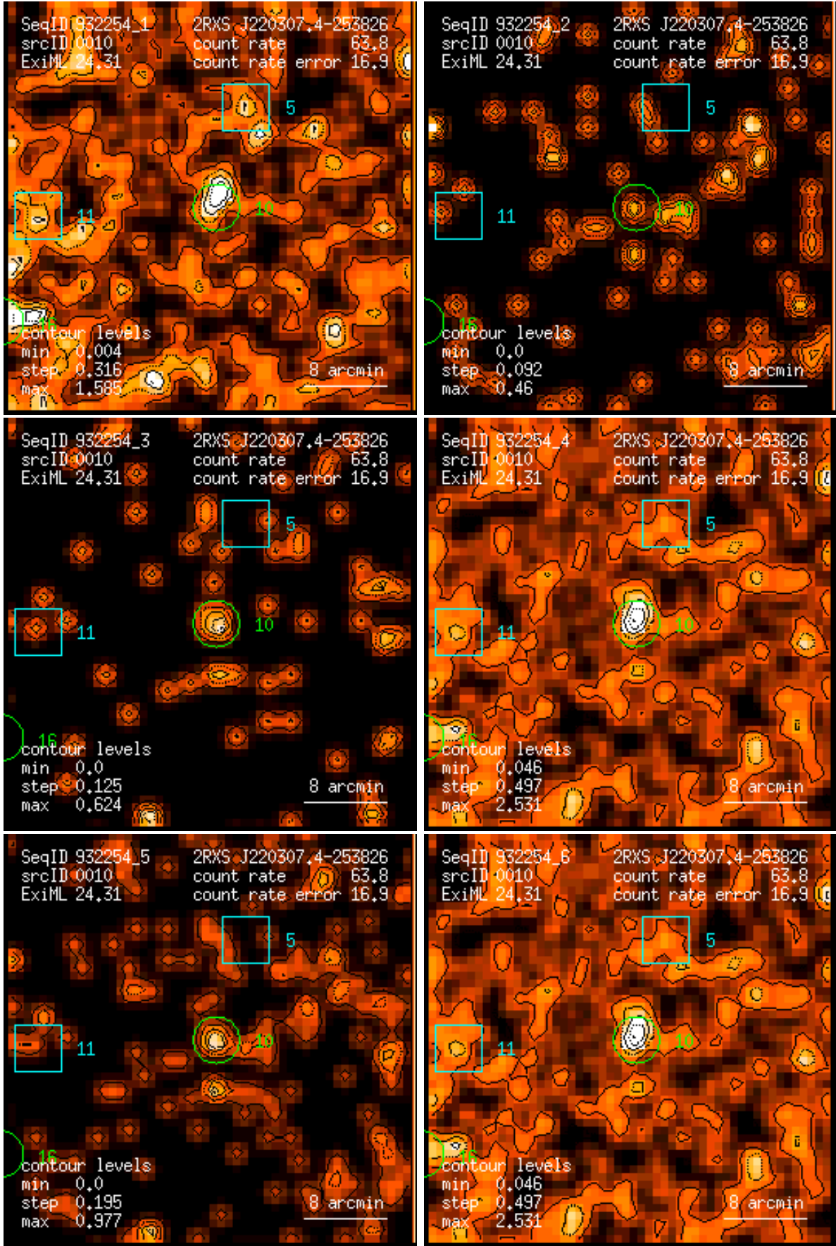
Figure 10: RASS 932254: detection 0010: band rate images, Gaussian filter: (1) PSPC channels 11 – 41, (2) 52 – 90, (3) 91 – 201, (4) 11 – 235, (5) 52 – 201, (6) 11 – 201. Broad band rates in counts/ks. Band rate contour levels in counts/ks/arcmin 2 .
