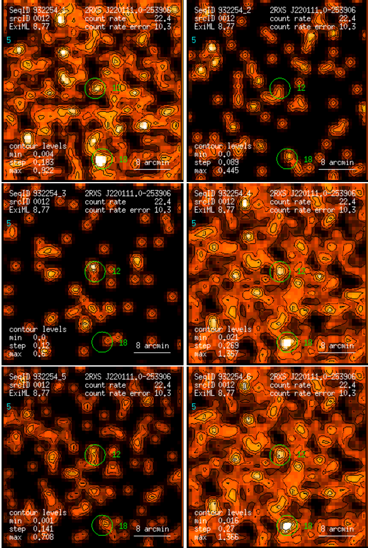
Figure 12: RASS 932254: detection 0012: band rate images, Gaussian filter: (1) PSPC channels 11 – 41, (2) 52 – 90, (3) 91 – 201, (4) 11 – 235, (5) 52 – 201, (6) 11 – 201. Broad band rates in counts/ks. Band rate contour levels in counts/ks/arcmin 2 .
