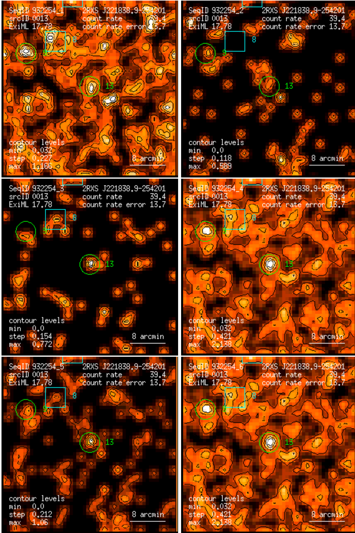
Figure 13: RASS 932254: detection 0013: band rate images, Gaussian filter: (1) PSPC channels 11 – 41, (2) 52 – 90, (3) 91 – 201, (4) 11 – 235, (5) 52 – 201, (6) 11 – 201. Broad band rates in counts/ks. Band rate contour levels in counts/ks/arcmin 2 .
