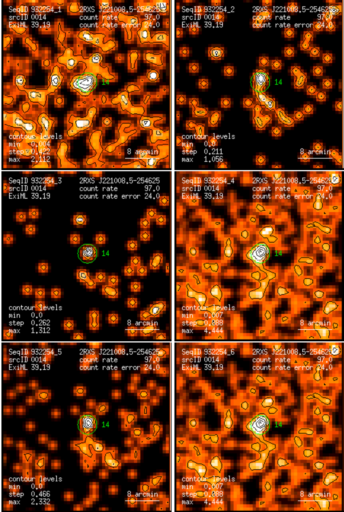
Figure 14: RASS 932254: detection 0014: band rate images, Gaussian filter: (1) PSPC channels 11 – 41, (2) 52 – 90, (3) 91 – 201, (4) 11 – 235, (5) 52 – 201, (6) 11 – 201. Broad band rates in counts/ks. Band rate contour levels in counts/ks/arcmin 2 .
