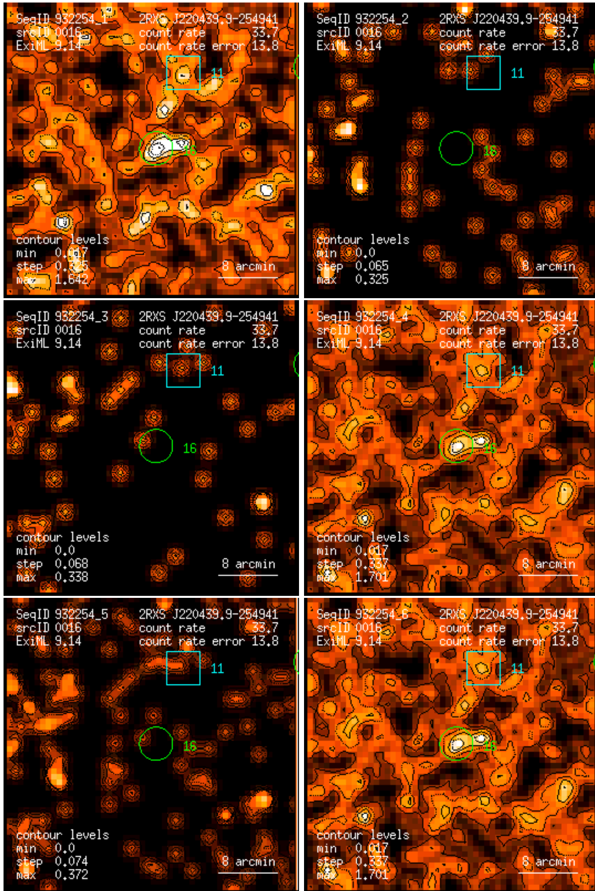
Figure 16: RASS 932254: detection 0016: band rate images, Gaussian filter: (1) PSPC channels 11 – 41, (2) 52 – 90, (3) 91 – 201, (4) 11 – 235, (5) 52 – 201, (6) 11 – 201. Broad band rates in counts/ks. Band rate contour levels in counts/ks/arcmin 2 .
