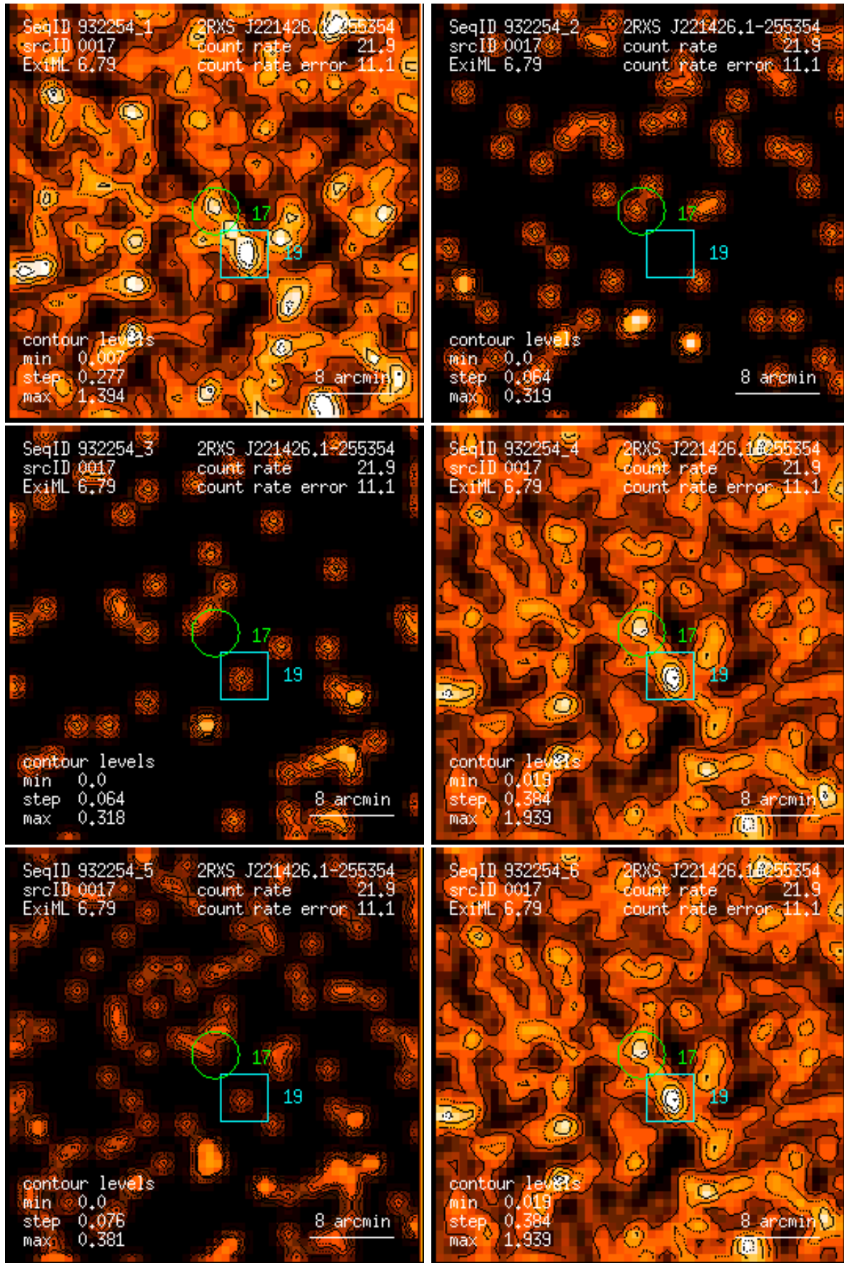
Figure 17: RASS 932254: detection 0017: band rate images, Gaussian filter: (1) PSPC channels 11 – 41, (2) 52 – 90, (3) 91 – 201, (4) 11 – 235, (5) 52 – 201, (6) 11 – 201. Broad band rates in counts/ks. Band rate contour levels in counts/ks/arcmin 2 .
