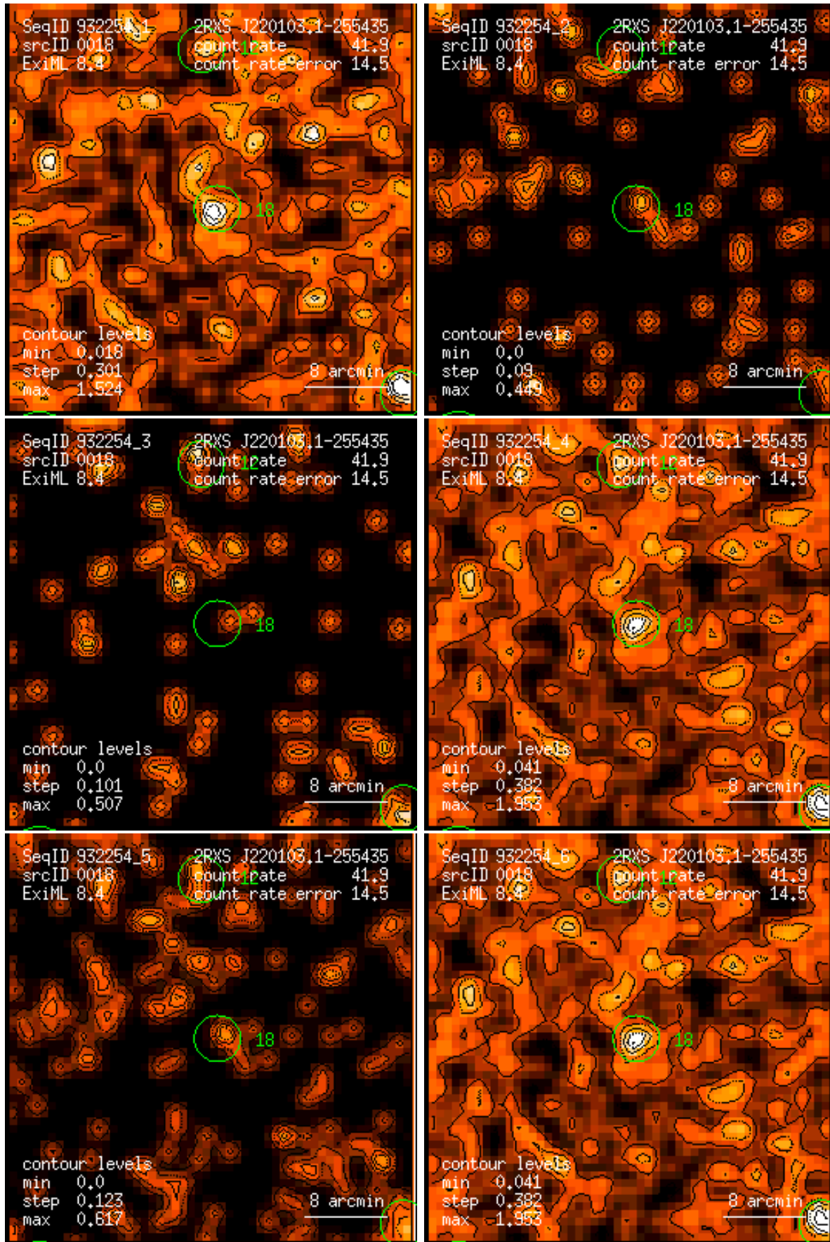
Figure 18: RASS 932254: detection 0018: band rate images, Gaussian filter: (1) PSPC channels 11 – 41, (2) 52 – 90, (3) 91 – 201, (4) 11 – 235, (5) 52 – 201, (6) 11 – 201. Broad band rates in counts/ks. Band rate contour levels in counts/ks/arcmin 2 .
