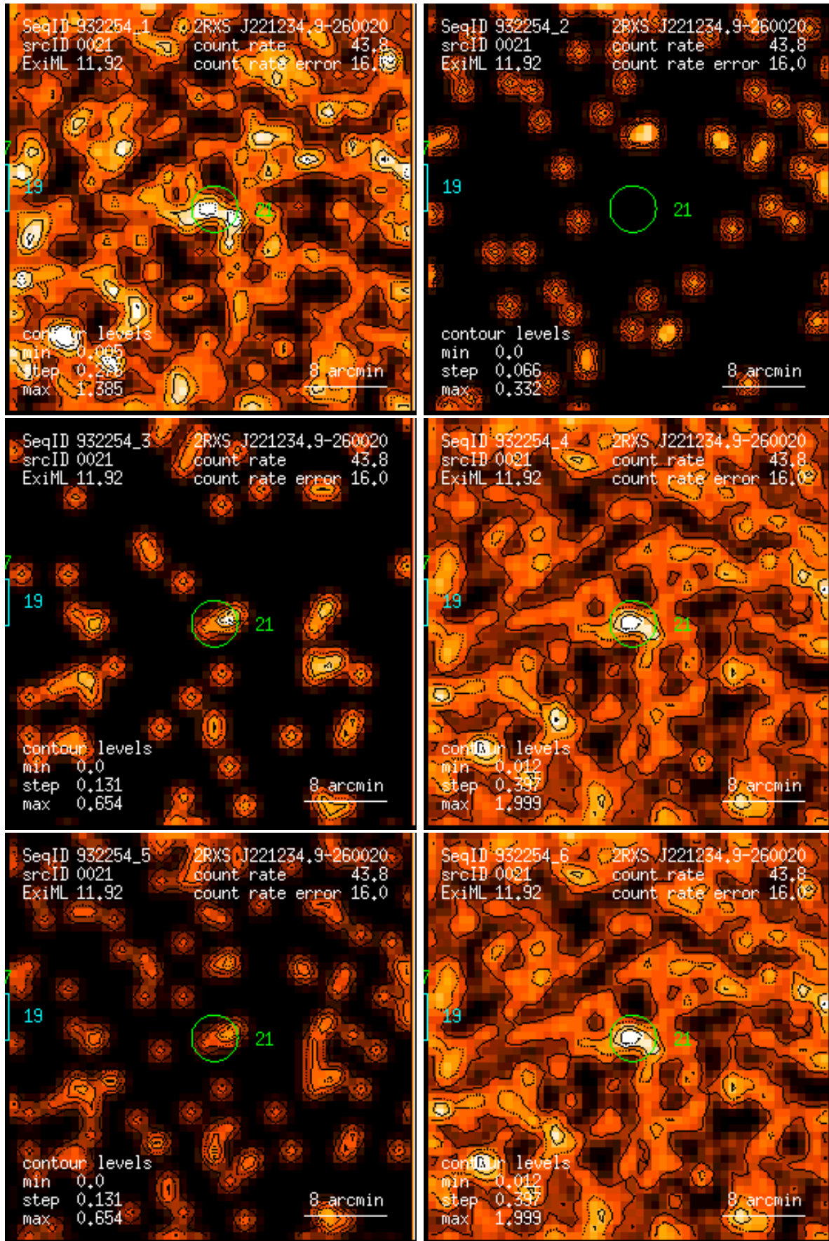
Figure 21: RASS 932254: detection 0021: band rate images, Gaussian filter: (1) PSPC channels 11 – 41, (2) 52 – 90, (3) 91 – 201, (4) 11 – 235, (5) 52 – 201, (6) 11 – 201. Broad band rates in counts/ks. Band rate contour levels in counts/ks/arcmin 2 .
