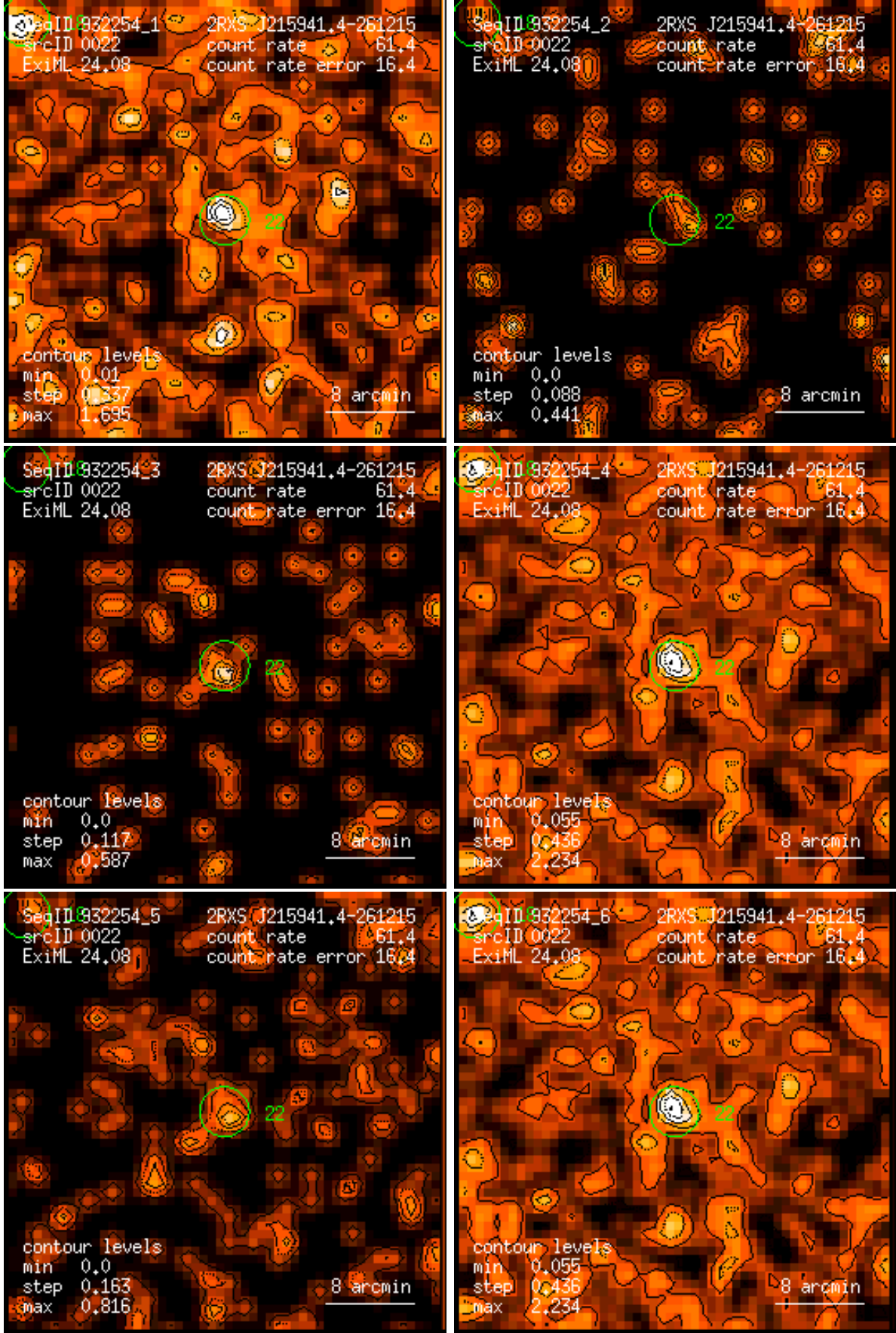
Figure 22: RASS 932254: detection 0022: band rate images, Gaussian filter: (1) PSPC channels 11 – 41, (2) 52 – 90, (3) 91 – 201, (4) 11 – 235, (5) 52 – 201, (6) 11 – 201. Broad band rates in counts/ks. Band rate contour levels in counts/ks/arcmin 2 .
