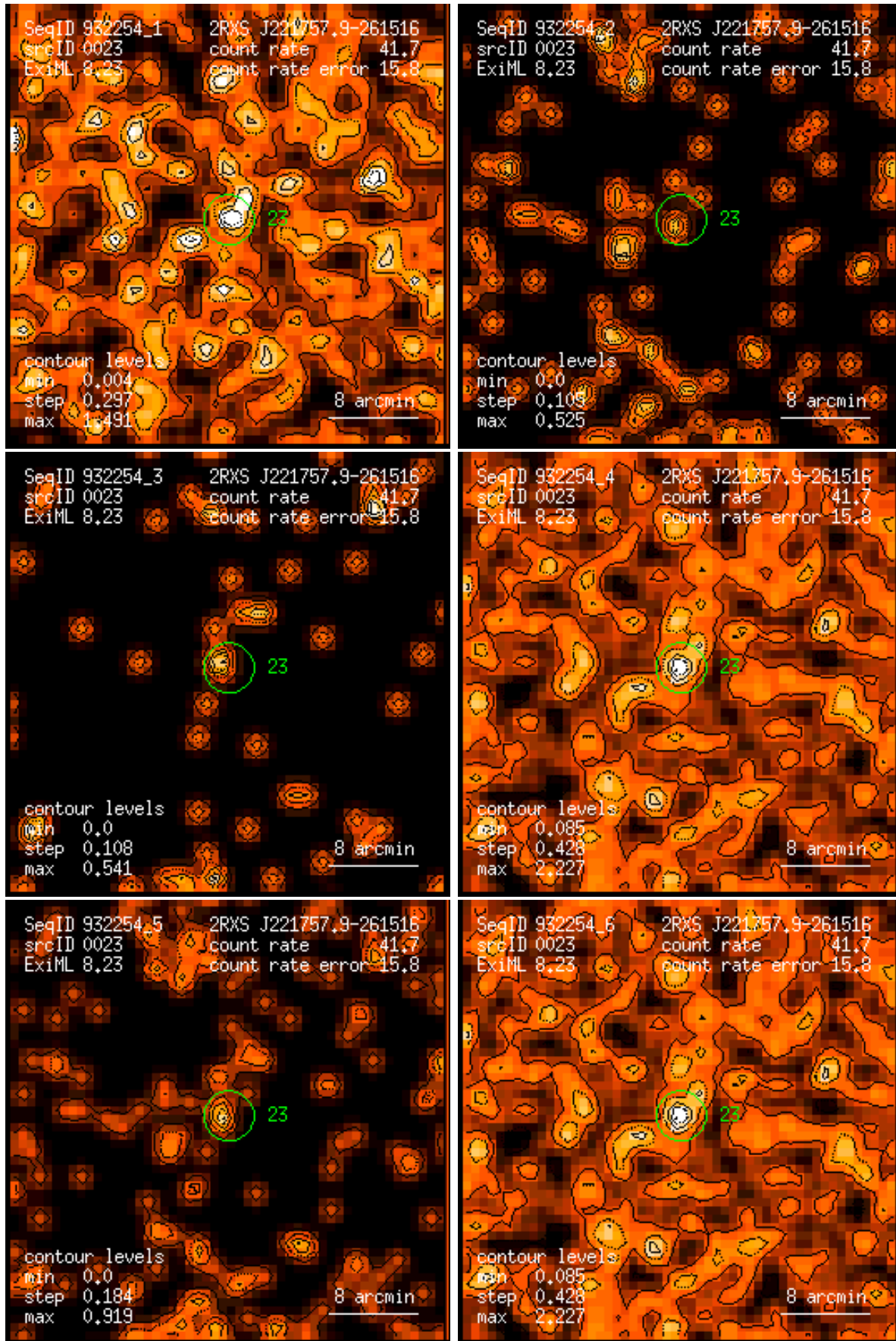
Figure 23: RASS 932254: detection 0023: band rate images, Gaussian filter: (1) PSPC channels 11 – 41, (2) 52 – 90, (3) 91 – 201, (4) 11 – 235, (5) 52 – 201, (6) 11 – 201. Broad band rates in counts/ks. Band rate contour levels in counts/ks/arcmin 2 .
