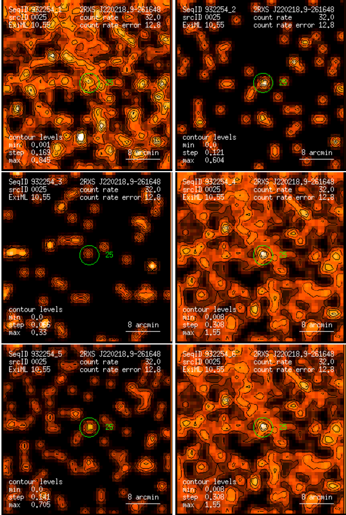
Figure 25: RASS 932254: detection 0025: band rate images, Gaussian filter: (1) PSPC channels 11 – 41, (2) 52 – 90, (3) 91 – 201, (4) 11 – 235, (5) 52 – 201, (6) 11 – 201. Broad band rates in counts/ks. Band rate contour levels in counts/ks/arcmin 2 .
