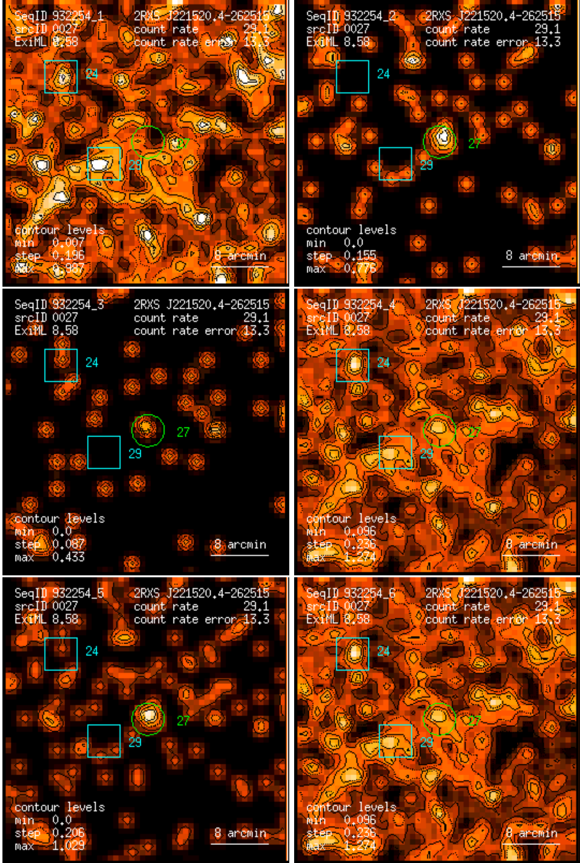
Figure 27: RASS 932254: detection 0027: band rate images, Gaussian filter: (1) PSPC channels 11 – 41, (2) 52 – 90, (3) 91 – 201, (4) 11 – 235, (5) 52 – 201, (6) 11 – 201. Broad band rates in counts/ks. Band rate contour levels in counts/ks/arcmin 2 .
