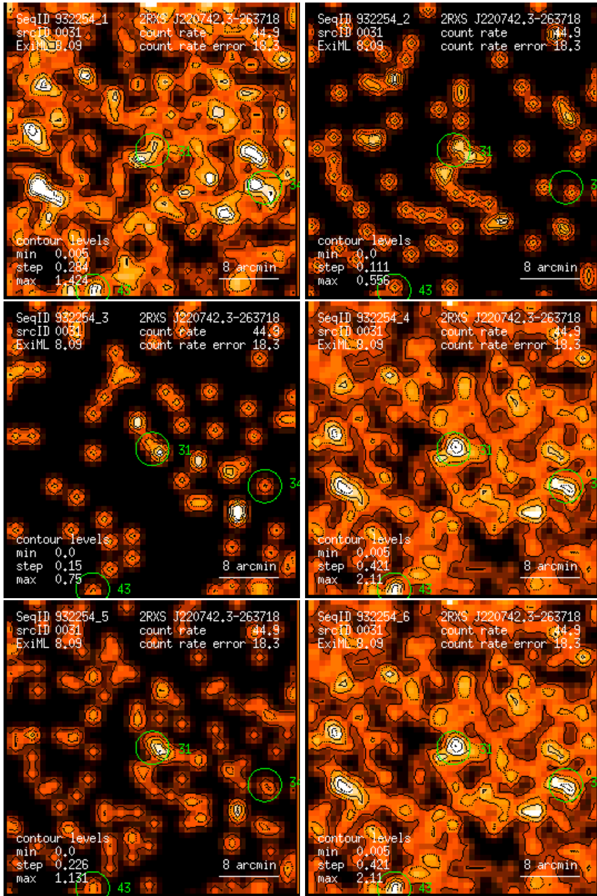
Figure 31: RASS 932254: detection 0031: band rate images, Gaussian filter: (1) PSPC channels 11 – 41, (2) 52 – 90, (3) 91 – 201, (4) 11 – 235, (5) 52 – 201, (6) 11 – 201. Broad band rates in counts/ks. Band rate contour levels in counts/ks/arcmin 2 .
