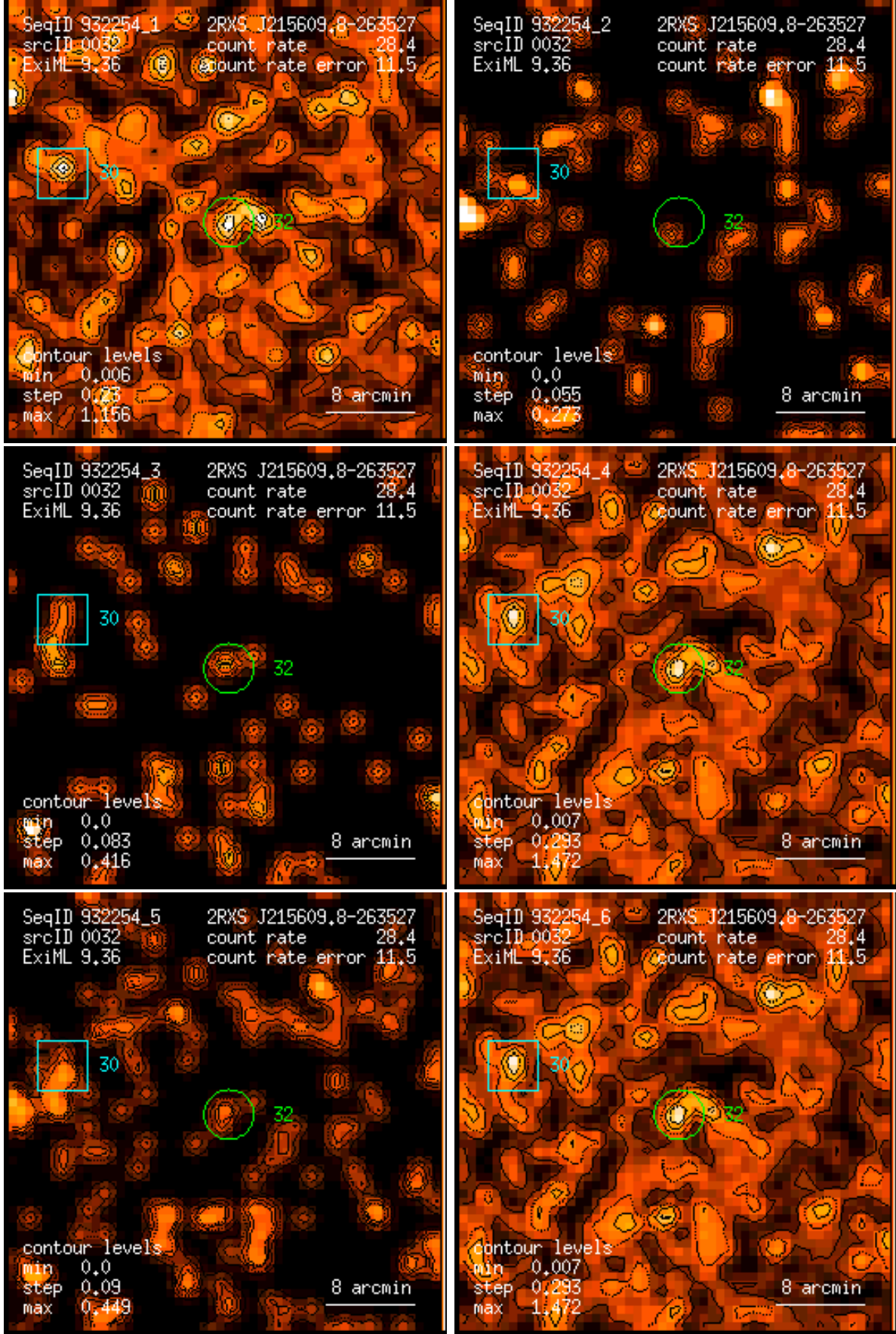
Figure 32: RASS 932254: detection 0032: band rate images, Gaussian filter: (1) PSPC channels 11 – 41, (2) 52 – 90, (3) 91 – 201, (4) 11 – 235, (5) 52 – 201, (6) 11 – 201. Broad band rates in counts/ks. Band rate contour levels in counts/ks/arcmin 2 .
