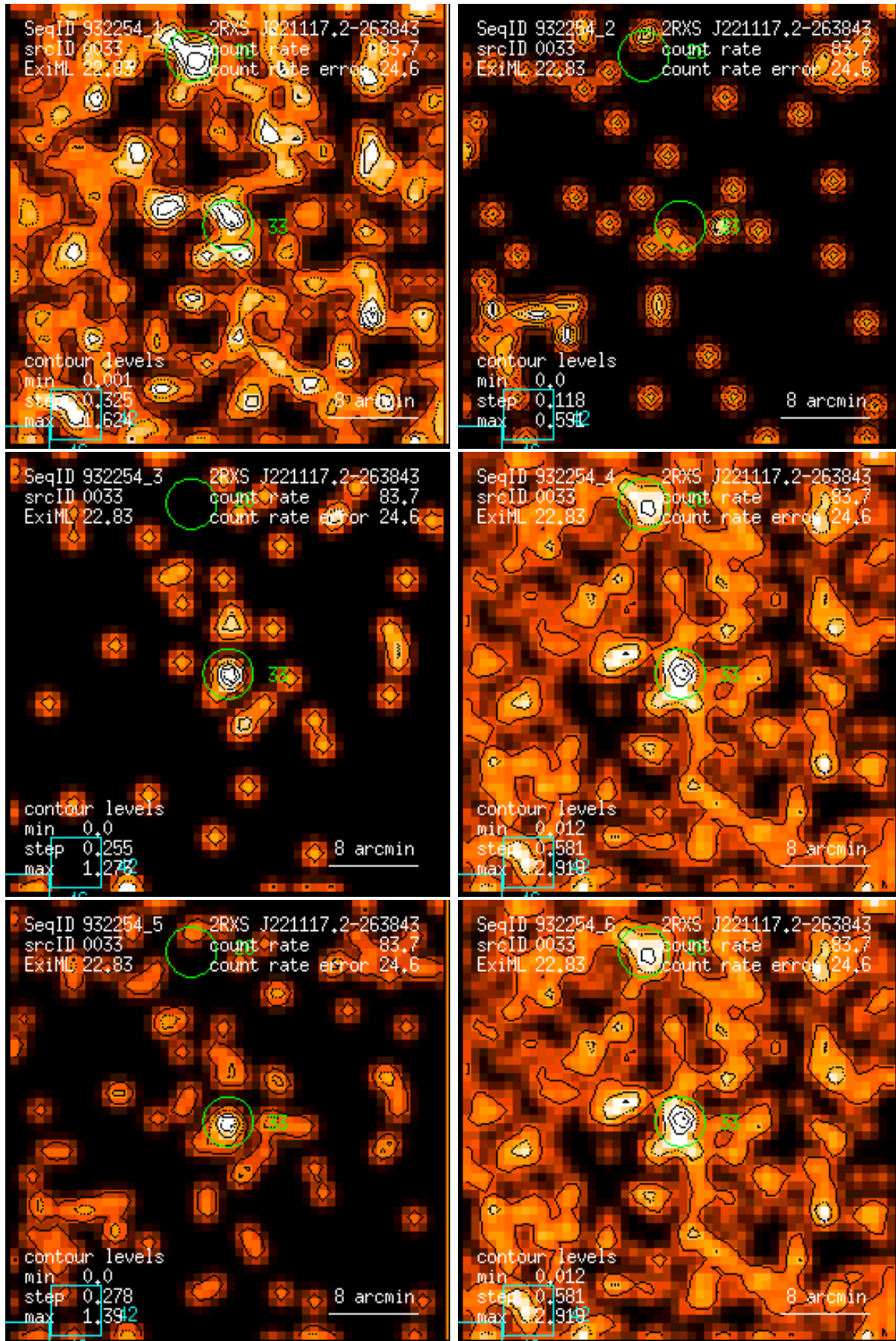
Figure 33: RASS 932254: detection 0033: band rate images, Gaussian filter: (1) PSPC channels 11 – 41, (2) 52 – 90, (3) 91 – 201, (4) 11 – 235, (5) 52 – 201, (6) 11 – 201. Broad band rates in counts/ks. Band rate contour levels in counts/ks/arcmin 2 .
