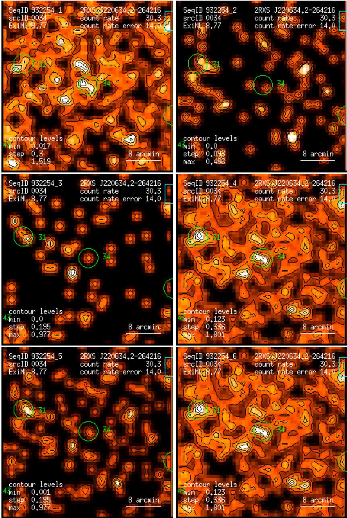
Figure 34: RASS 932254: detection 0034: band rate images, Gaussian filter: (1) PSPC channels 11 – 41, (2) 52 – 90, (3) 91 – 201, (4) 11 – 235, (5) 52 – 201, (6) 11 – 201. Broad band rates in counts/ks. Band rate contour levels in counts/ks/arcmin 2 .
