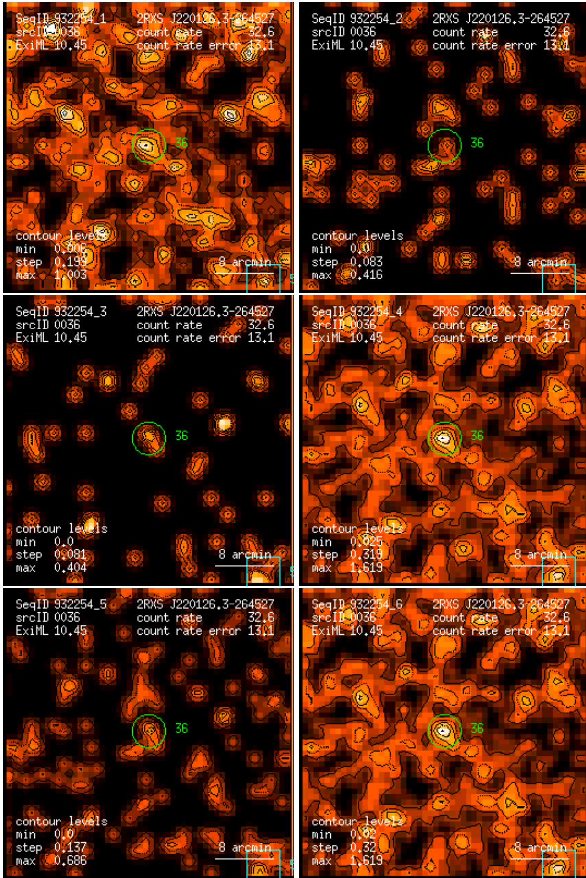
Figure 36: RASS 932254: detection 0036: band rate images, Gaussian filter: (1) PSPC channels 11 – 41, (2) 52 – 90, (3) 91 – 201, (4) 11 – 235, (5) 52 – 201, (6) 11 – 201. Broad band rates in counts/ks. Band rate contour levels in counts/ks/arcmin 2 .
