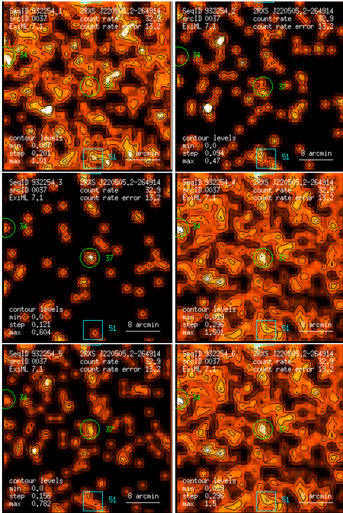
Figure 37: RASS 932254: detection 0037: band rate images, Gaussian filter: (1) PSPC channels 11 – 41, (2) 52 – 90, (3) 91 – 201, (4) 11 – 235, (5) 52 – 201, (6) 11 – 201. Broad band rates in counts/ks. Band rate contour levels in counts/ks/arcmin 2 .
