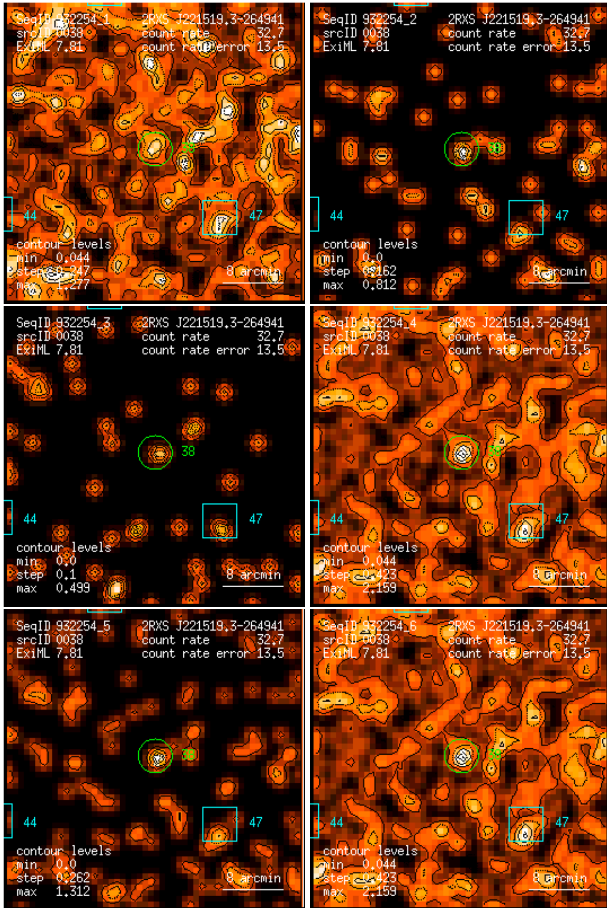
Figure 38: RASS 932254: detection 0038: band rate images, Gaussian filter: (1) PSPC channels 11 – 41, (2) 52 – 90, (3) 91 – 201, (4) 11 – 235, (5) 52 – 201, (6) 11 – 201. Broad band rates in counts/ks. Band rate contour levels in counts/ks/arcmin 2 .
