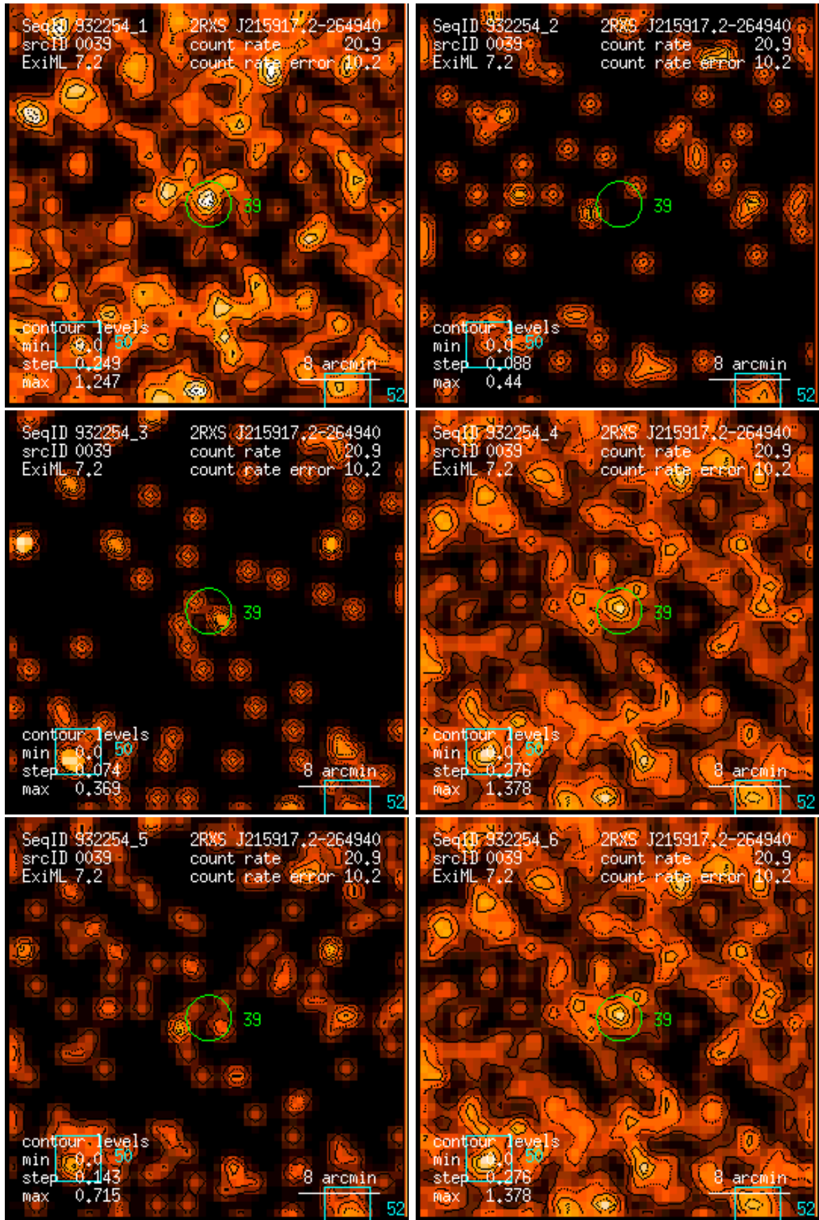
Figure 39: RASS 932254: detection 0039: band rate images, Gaussian filter: (1) PSPC channels 11 – 41, (2) 52 – 90, (3) 91 – 201, (4) 11 – 235, (5) 52 – 201, (6) 11 – 201. Broad band rates in counts/ks. Band rate contour levels in counts/ks/arcmin 2 .
