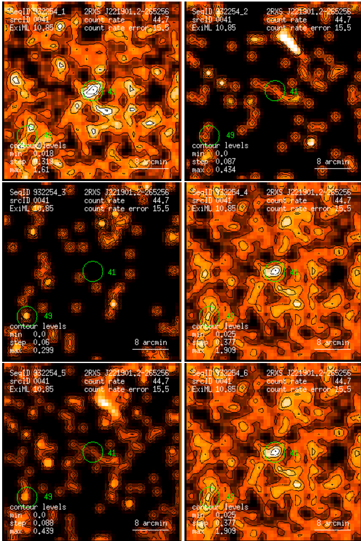
Figure 41: RASS 932254: detection 0041: band rate images, Gaussian filter: (1) PSPC channels 11 – 41, (2) 52 – 90, (3) 91 – 201, (4) 11 – 235, (5) 52 – 201, (6) 11 – 201. Broad band rates in counts/ks. Band rate contour levels in counts/ks/arcmin 2 .
