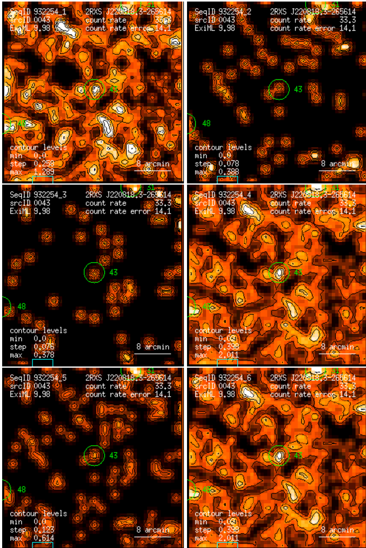
Figure 43: RASS 932254: detection 0043: band rate images, Gaussian filter: (1) PSPC channels 11 – 41, (2) 52 – 90, (3) 91 – 201, (4) 11 – 235, (5) 52 – 201, (6) 11 – 201. Broad band rates in counts/ks. Band rate contour levels in counts/ks/arcmin 2 .
