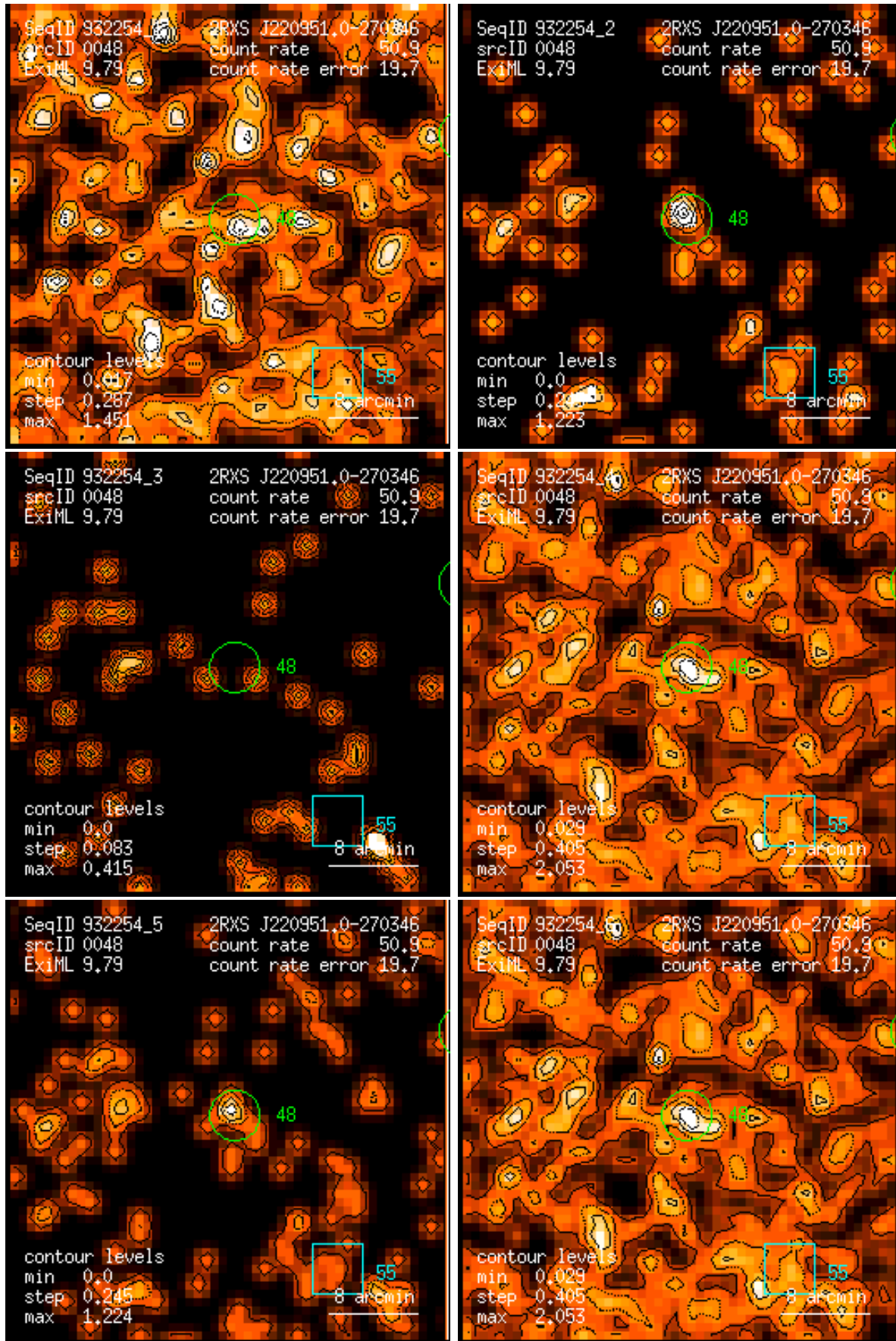
Figure 48: RASS 932254: detection 0048: band rate images, Gaussian filter: (1) PSPC channels 11 – 41, (2) 52 – 90, (3) 91 – 201, (4) 11 – 235, (5) 52 – 201, (6) 11 – 201. Broad band rates in counts/ks. Band rate contour levels in counts/ks/arcmin 2 .
