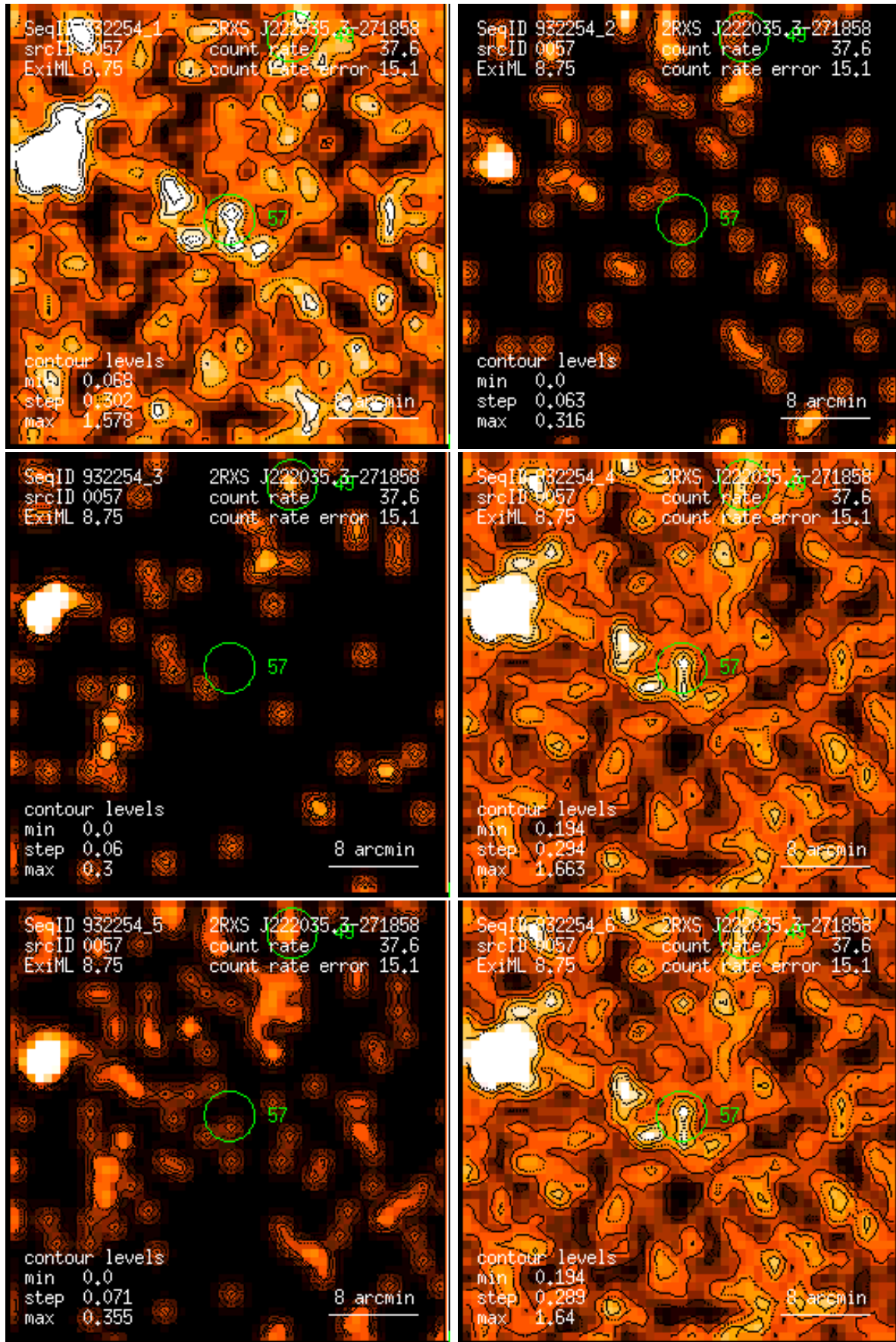
Figure 57: RASS 932254: detection 0057: band rate images, Gaussian filter: (1) PSPC channels 11 – 41, (2) 52 – 90, (3) 91 – 201, (4) 11 – 235, (5) 52 – 201, (6) 11 – 201. Broad band rates in counts/ks. Band rate contour levels in counts/ks/arcmin 2 .
