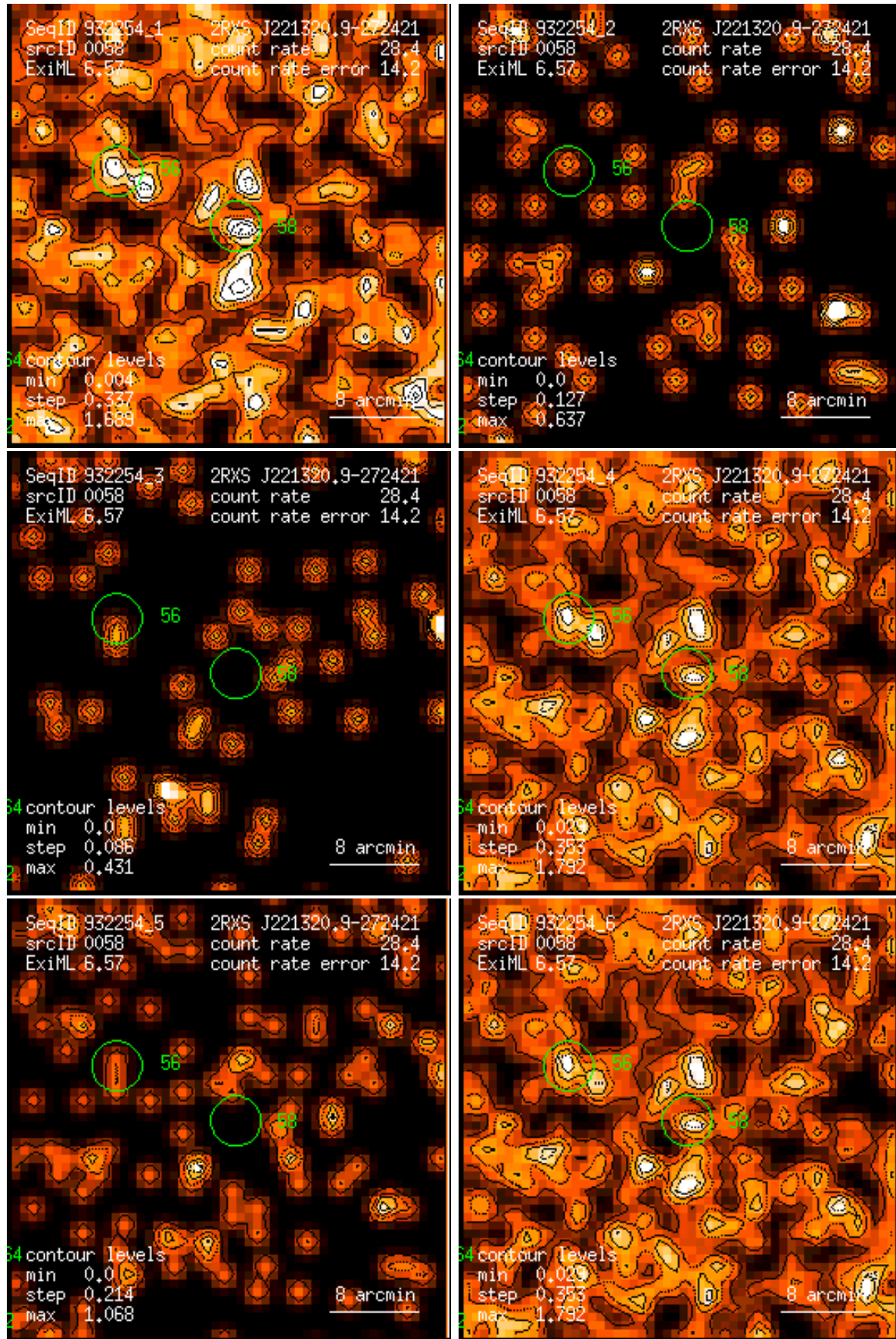
Figure 58: RASS 932254: detection 0058: band rate images, Gaussian filter: (1) PSPC channels 11 – 41, (2) 52 – 90, (3) 91 – 201, (4) 11 – 235, (5) 52 – 201, (6) 11 – 201. Broad band rates in counts/ks. Band rate contour levels in counts/ks/arcmin 2 .
