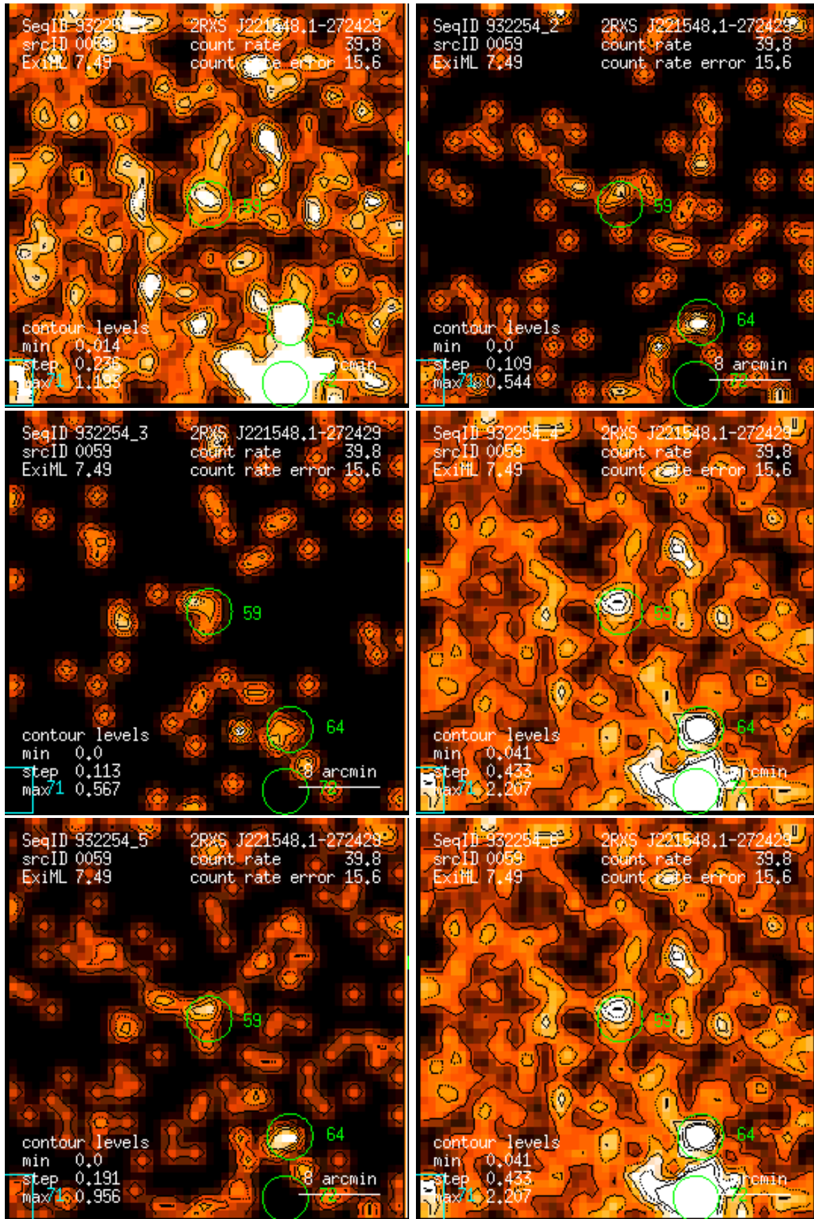
Figure 59: RASS 932254: detection 0059: band rate images, Gaussian filter: (1) PSPC channels 11 – 41, (2) 52 – 90, (3) 91 – 201, (4) 11 – 235, (5) 52 – 201, (6) 11 – 201. Broad band rates in counts/ks. Band rate contour levels in counts/ks/arcmin 2 .
