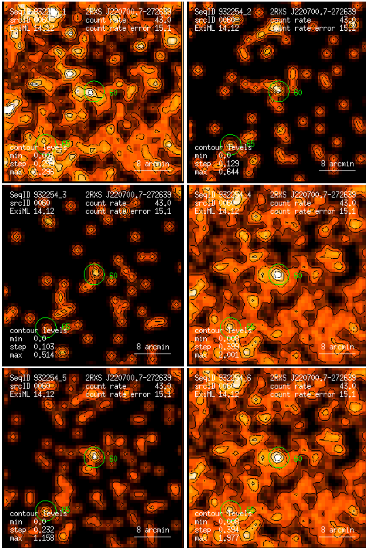
Figure 60: RASS 932254: detection 0060: band rate images, Gaussian filter: (1) PSPC channels 11 – 41, (2) 52 – 90, (3) 91 – 201, (4) 11 – 235, (5) 52 – 201, (6) 11 – 201. Broad band rates in counts/ks. Band rate contour levels in counts/ks/arcmin 2 .
