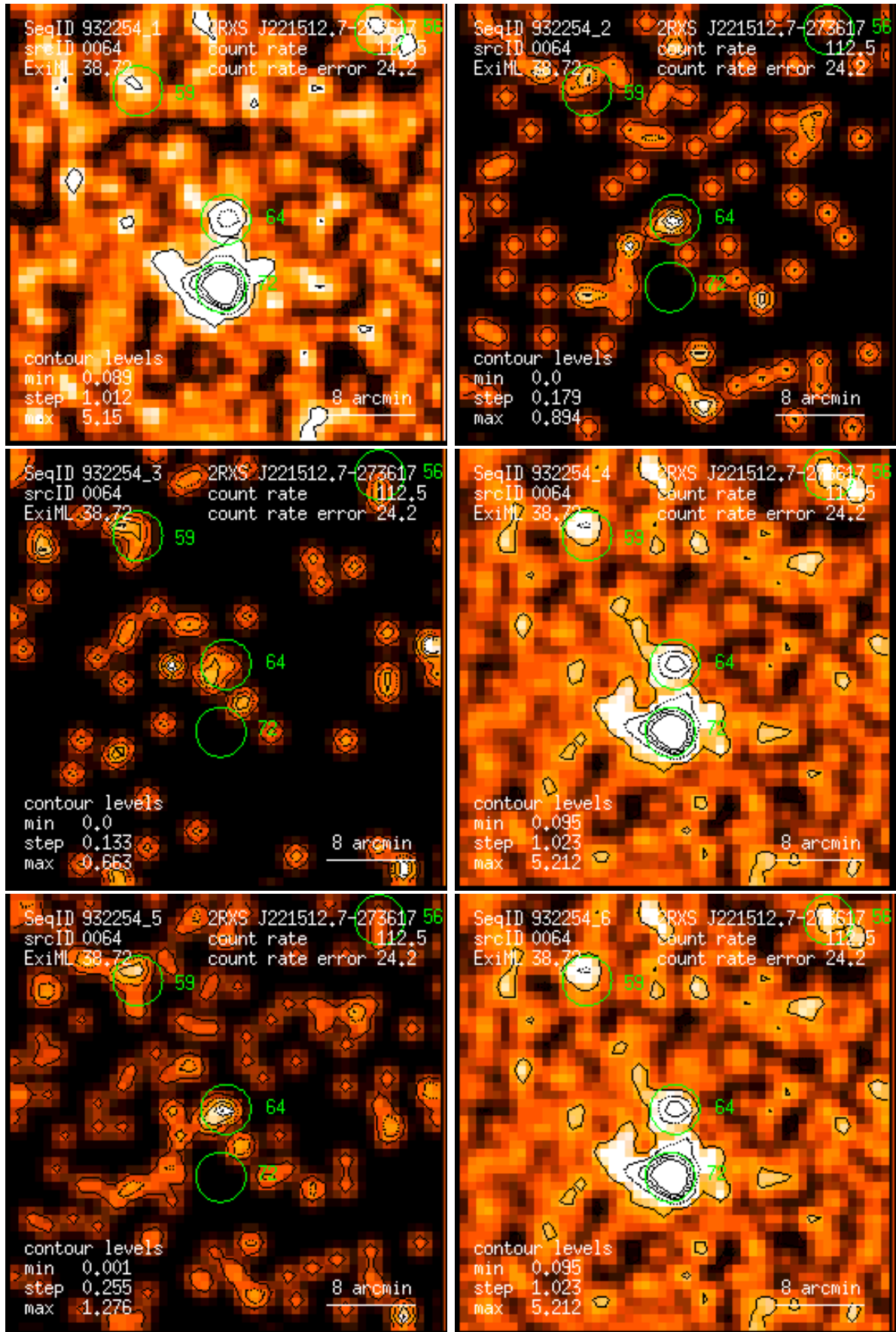
Figure 64: RASS 932254: detection 0064: band rate images, Gaussian filter: (1) PSPC channels 11 – 41, (2) 52 – 90, (3) 91 – 201, (4) 11 – 235, (5) 52 – 201, (6) 11 – 201. Broad band rates in counts/ks. Band rate contour levels in counts/ks/arcmin 2 .
