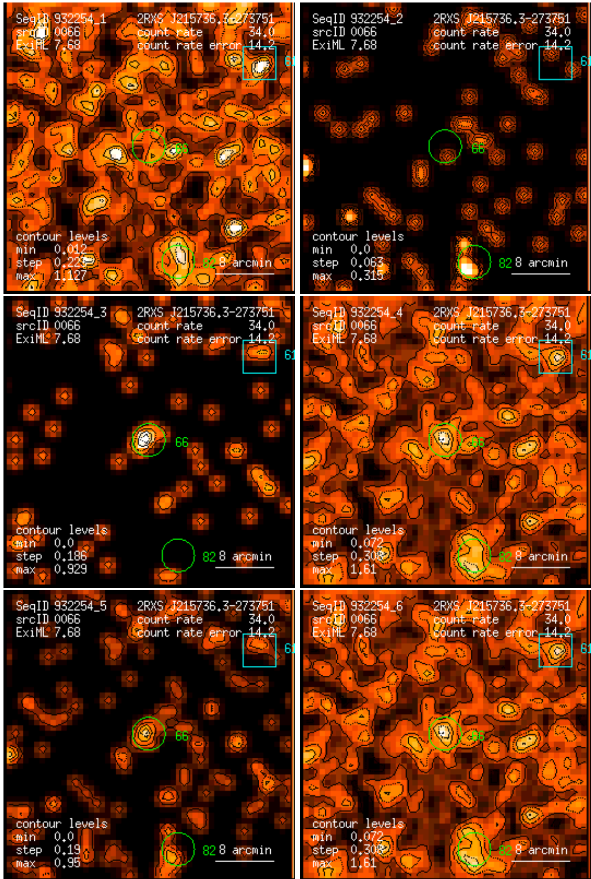
Figure 66: RASS 932254: detection 0066: band rate images, Gaussian filter: (1) PSPC channels 11 – 41, (2) 52 – 90, (3) 91 – 201, (4) 11 – 235, (5) 52 – 201, (6) 11 – 201. Broad band rates in counts/ks. Band rate contour levels in counts/ks/arcmin 2 .
