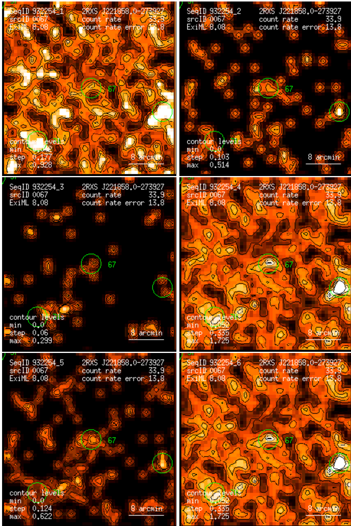
Figure 67: RASS 932254: detection 0067: band rate images, Gaussian filter: (1) PSPC channels 11 – 41, (2) 52 – 90, (3) 91 – 201, (4) 11 – 235, (5) 52 – 201, (6) 11 – 201. Broad band rates in counts/ks. Band rate contour levels in counts/ks/arcmin 2 .
