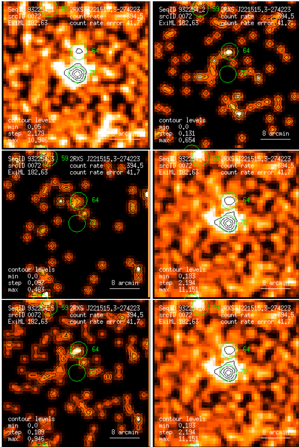
Figure 72: RASS 932254: detection 0072: band rate images, Gaussian filter: (1) PSPC channels 11 – 41, (2) 52 – 90, (3) 91 – 201, (4) 11 – 235, (5) 52 – 201, (6) 11 – 201. Broad band rates in counts/ks. Band rate contour levels in counts/ks/arcmin 2 .
