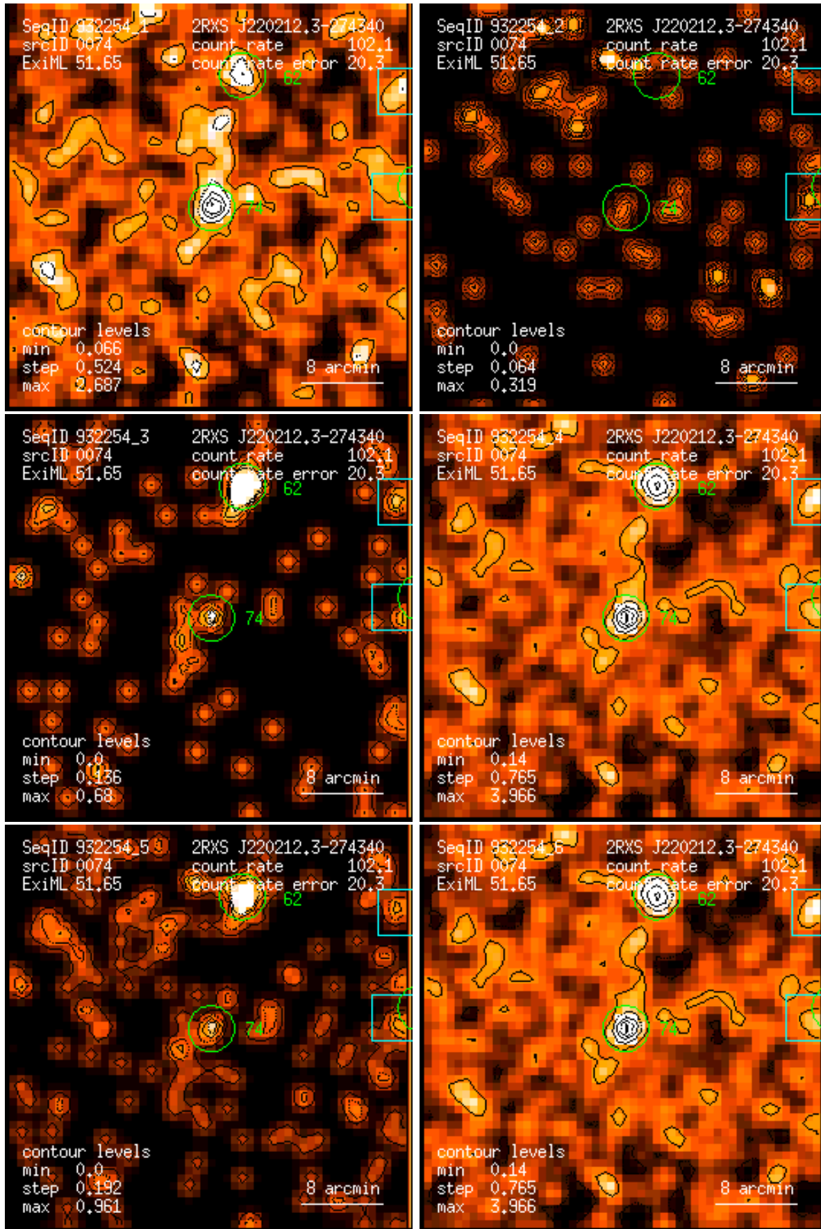
Figure 74: RASS 932254: detection 0074: band rate images, Gaussian filter: (1) PSPC channels 11 – 41, (2) 52 – 90, (3) 91 – 201, (4) 11 – 235, (5) 52 – 201, (6) 11 – 201. Broad band rates in counts/ks. Band rate contour levels in counts/ks/arcmin 2 .
