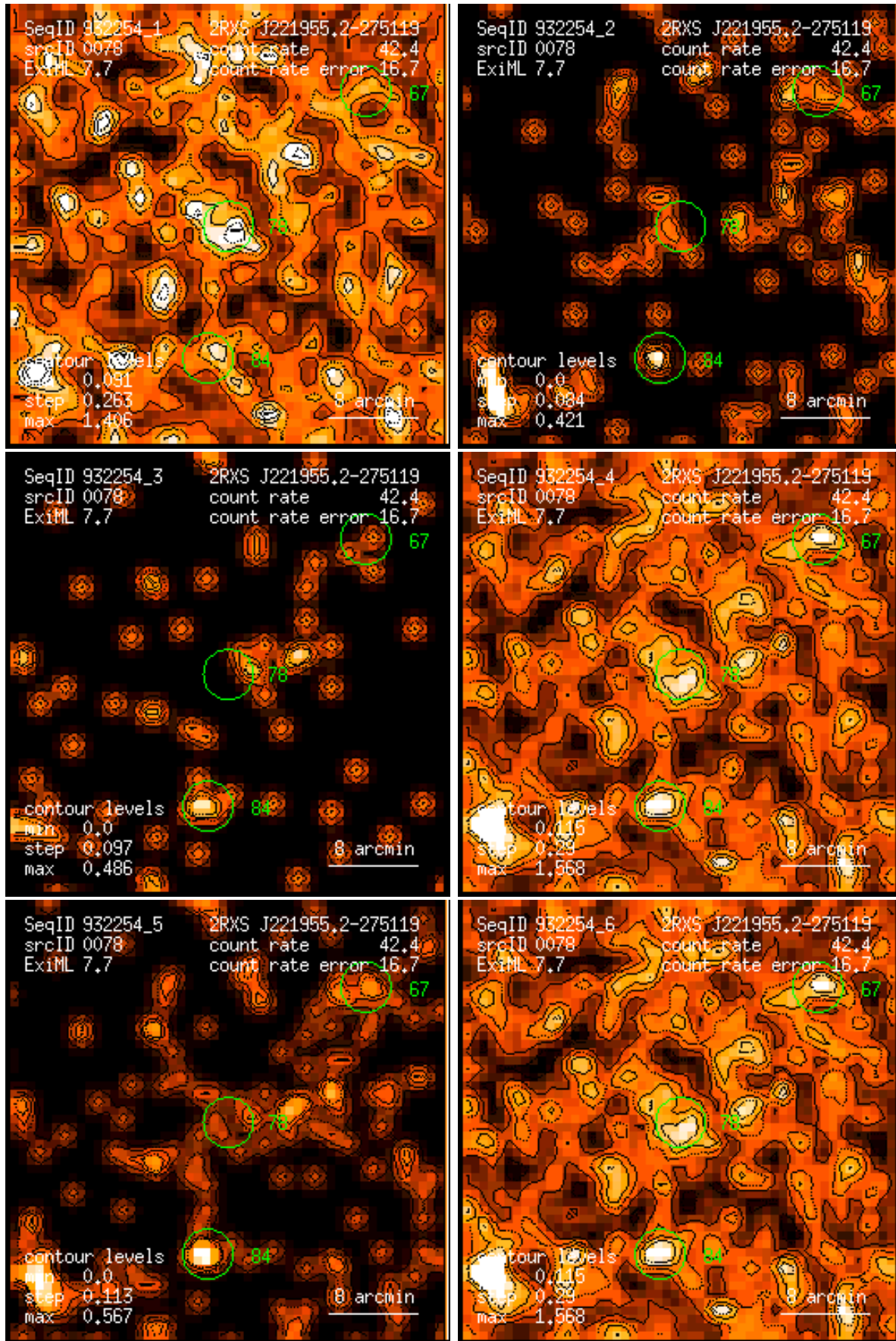
Figure 78: RASS 932254: detection 0078: band rate images, Gaussian filter: (1) PSPC channels 11 – 41, (2) 52 – 90, (3) 91 – 201, (4) 11 – 235, (5) 52 – 201, (6) 11 – 201. Broad band rates in counts/ks. Band rate contour levels in counts/ks/arcmin 2 .
