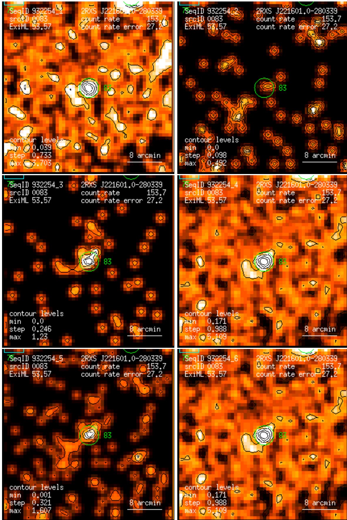
Figure 83: RASS 932254: detection 0083: band rate images, Gaussian filter: (1) PSPC channels 11 – 41, (2) 52 – 90, (3) 91 – 201, (4) 11 – 235, (5) 52 – 201, (6) 11 – 201. Broad band rates in counts/ks. Band rate contour levels in counts/ks/arcmin 2 .
