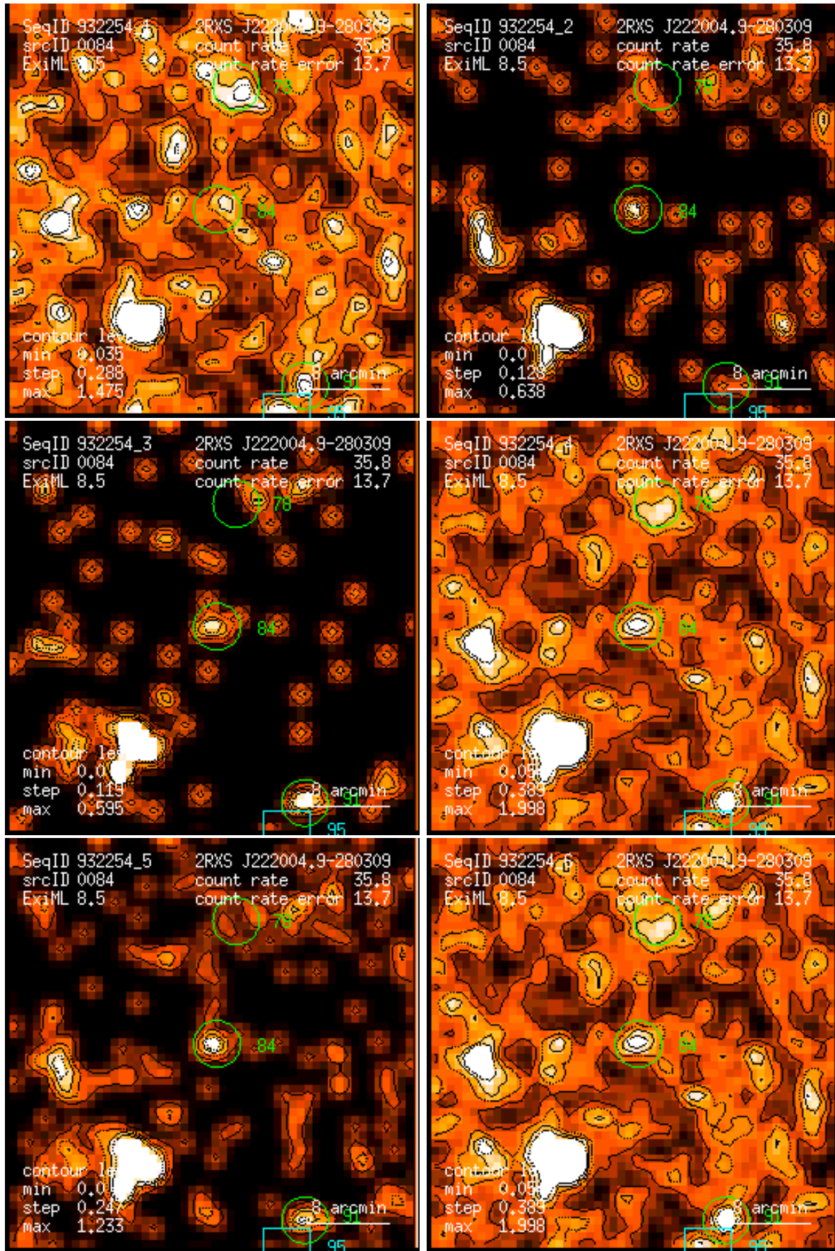
Figure 84: RASS 932254: detection 0084: band rate images, Gaussian filter: (1) PSPC channels 11 – 41, (2) 52 – 90, (3) 91 – 201, (4) 11 – 235, (5) 52 – 201, (6) 11 – 201. Broad band rates in counts/ks. Band rate contour levels in counts/ks/arcmin 2 .
