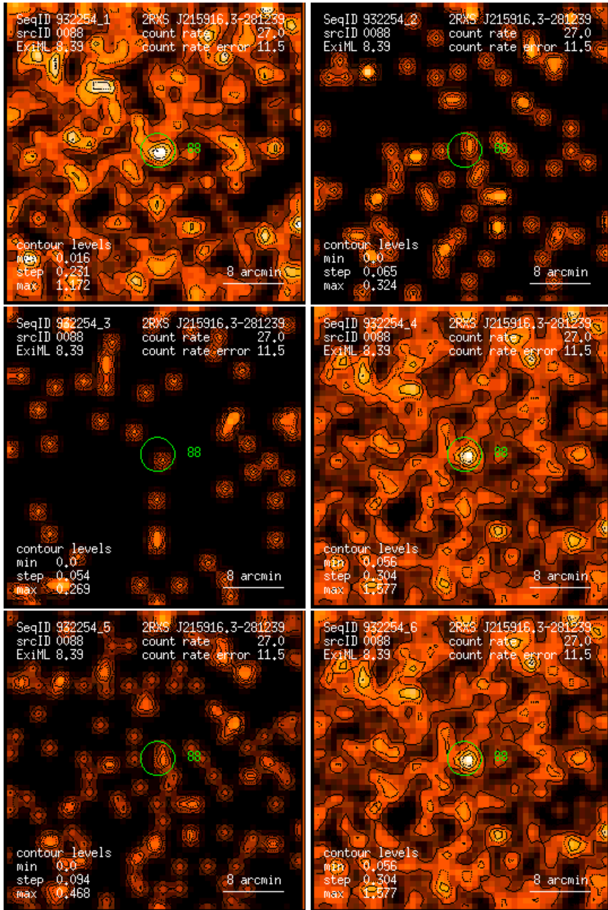
Figure 88: RASS 932254: detection 0088: band rate images, Gaussian filter: (1) PSPC channels 11 – 41, (2) 52 – 90, (3) 91 – 201, (4) 11 – 235, (5) 52 – 201, (6) 11 – 201. Broad band rates in counts/ks. Band rate contour levels in counts/ks/arcmin 2 .
