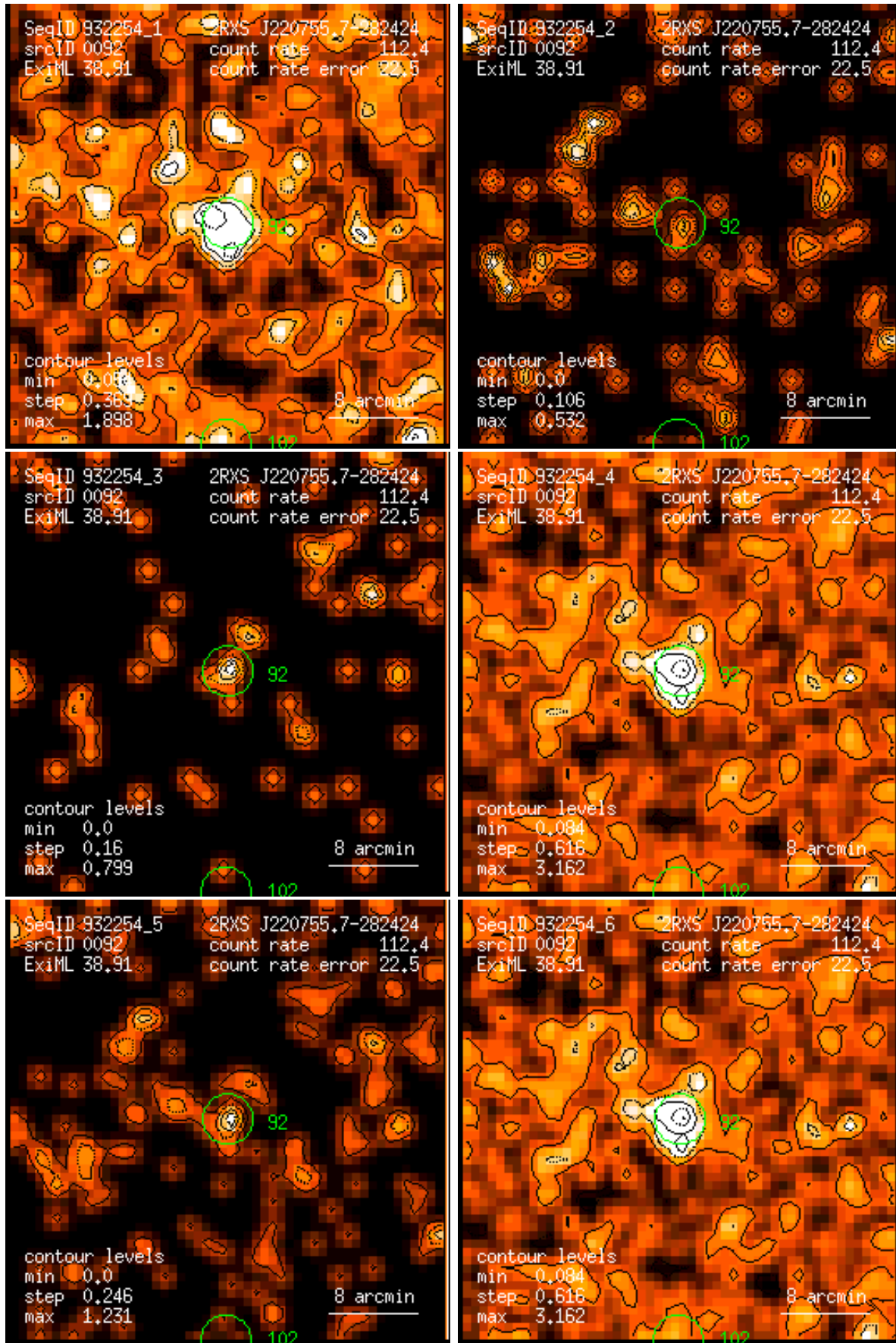
Figure 92: RASS 932254: detection 0092: band rate images, Gaussian filter: (1) PSPC channels 11 – 41, (2) 52 – 90, (3) 91 – 201, (4) 11 – 235, (5) 52 – 201, (6) 11 – 201. Broad band rates in counts/ks. Band rate contour levels in counts/ks/arcmin 2 .
