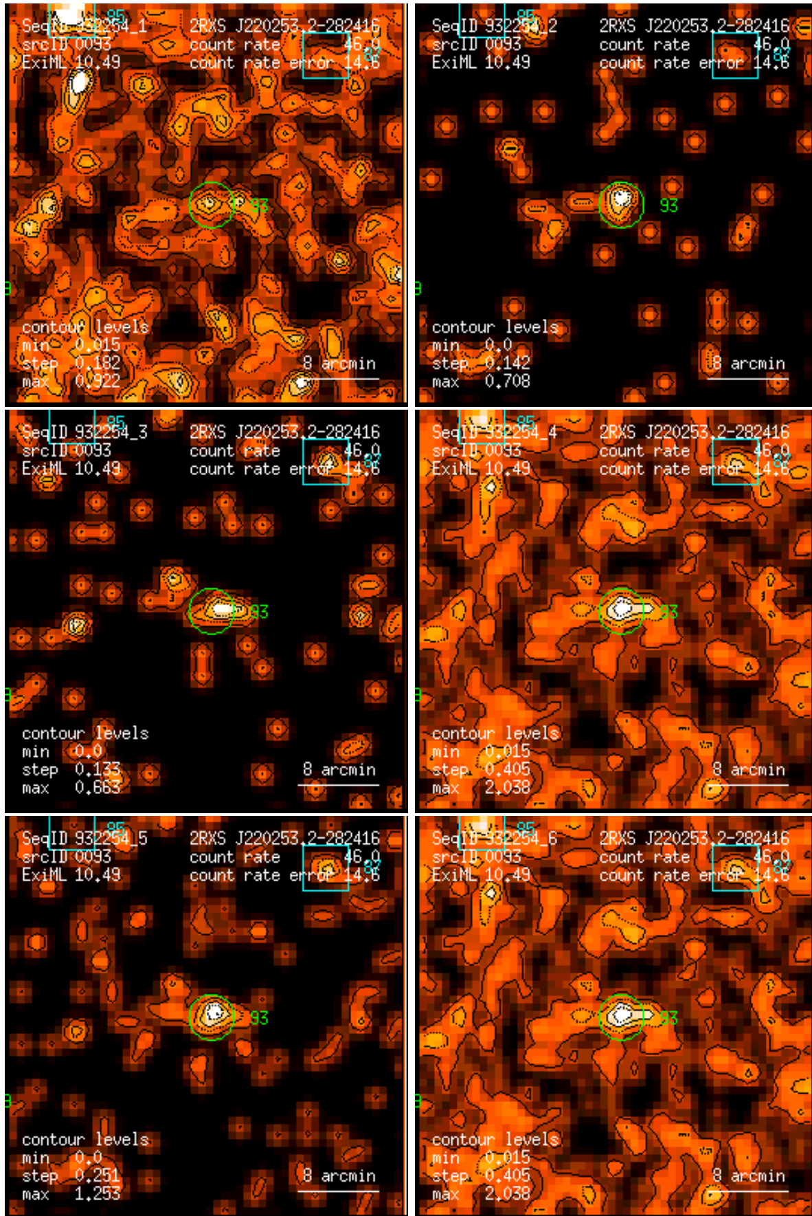
Figure 93: RASS 932254: detection 0093: band rate images, Gaussian filter: (1) PSPC channels 11 – 41, (2) 52 – 90, (3) 91 – 201, (4) 11 – 235, (5) 52 – 201, (6) 11 – 201. Broad band rates in counts/ks. Band rate contour levels in counts/ks/arcmin 2 .
