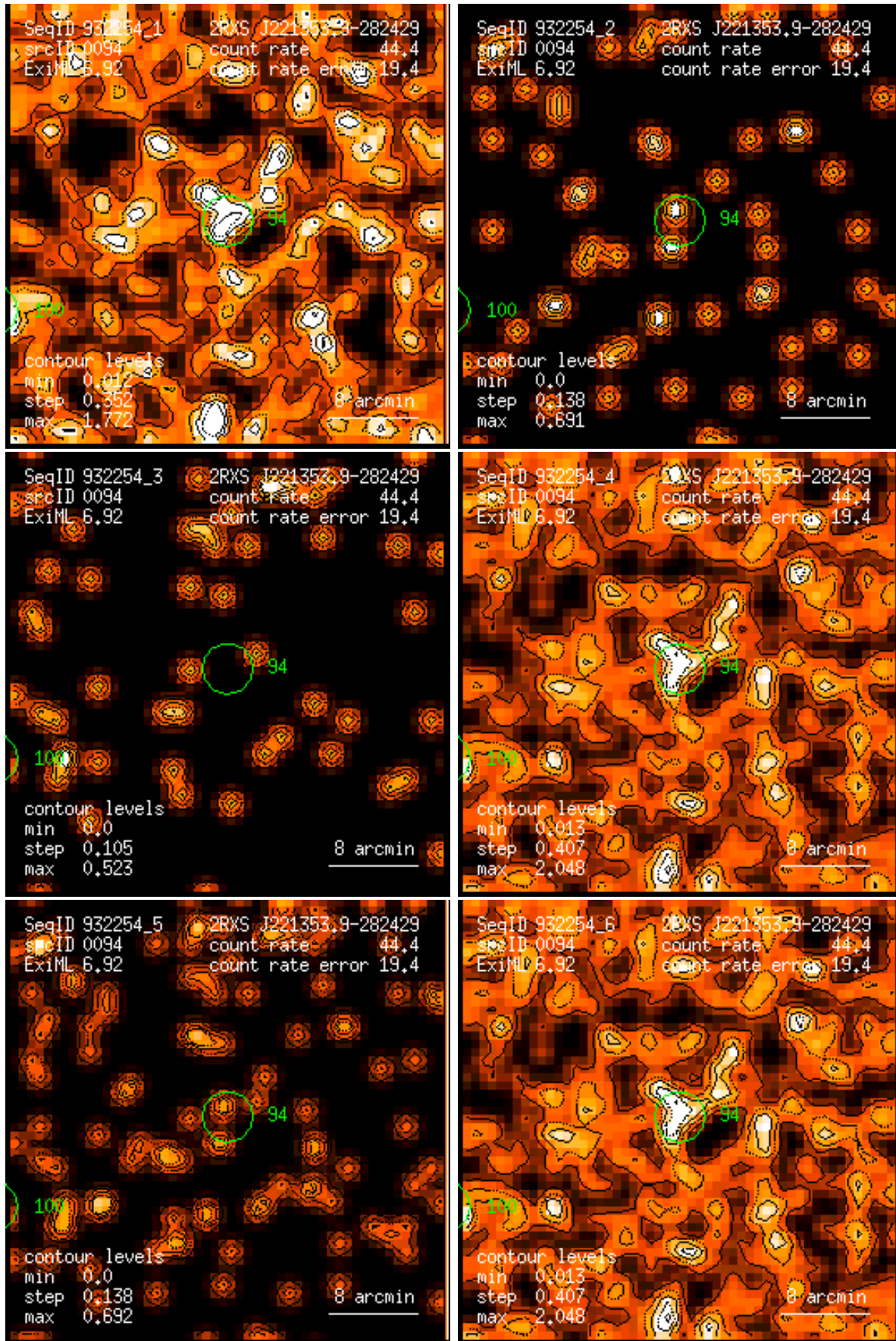
Figure 94: RASS 932254: detection 0094: band rate images, Gaussian filter: (1) PSPC channels 11 – 41, (2) 52 – 90, (3) 91 – 201, (4) 11 – 235, (5) 52 – 201, (6) 11 – 201. Broad band rates in counts/ks. Band rate contour levels in counts/ks/arcmin 2 .
