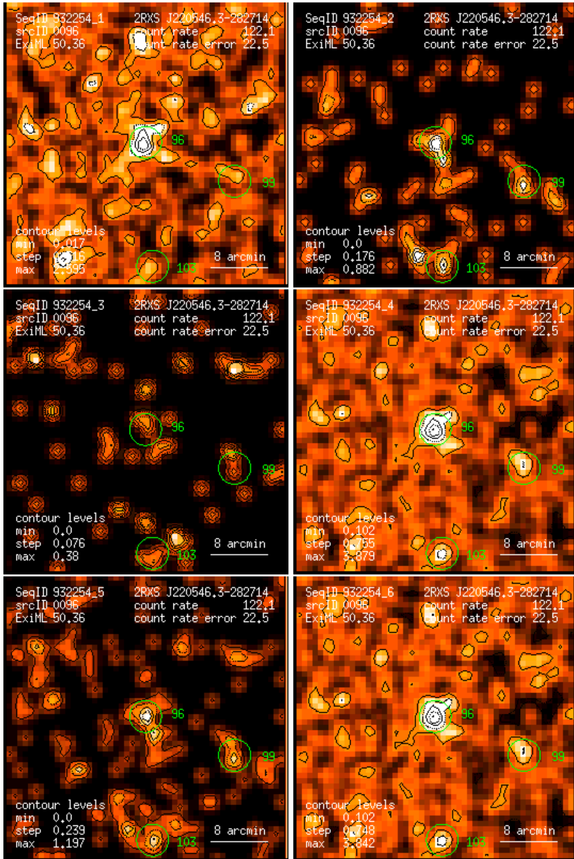
Figure 96: RASS 932254: detection 0096: band rate images, Gaussian filter: (1) PSPC channels 11 – 41, (2) 52 – 90, (3) 91 – 201, (4) 11 – 235, (5) 52 – 201, (6) 11 – 201. Broad band rates in counts/ks. Band rate contour levels in counts/ks/arcmin 2 .
