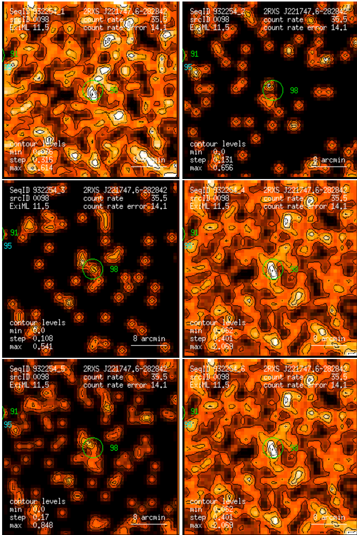
Figure 98: RASS 932254: detection 0098: band rate images, Gaussian filter: (1) PSPC channels 11 – 41, (2) 52 – 90, (3) 91 – 201, (4) 11 – 235, (5) 52 – 201, (6) 11 – 201. Broad band rates in counts/ks. Band rate contour levels in counts/ks/arcmin 2 .
