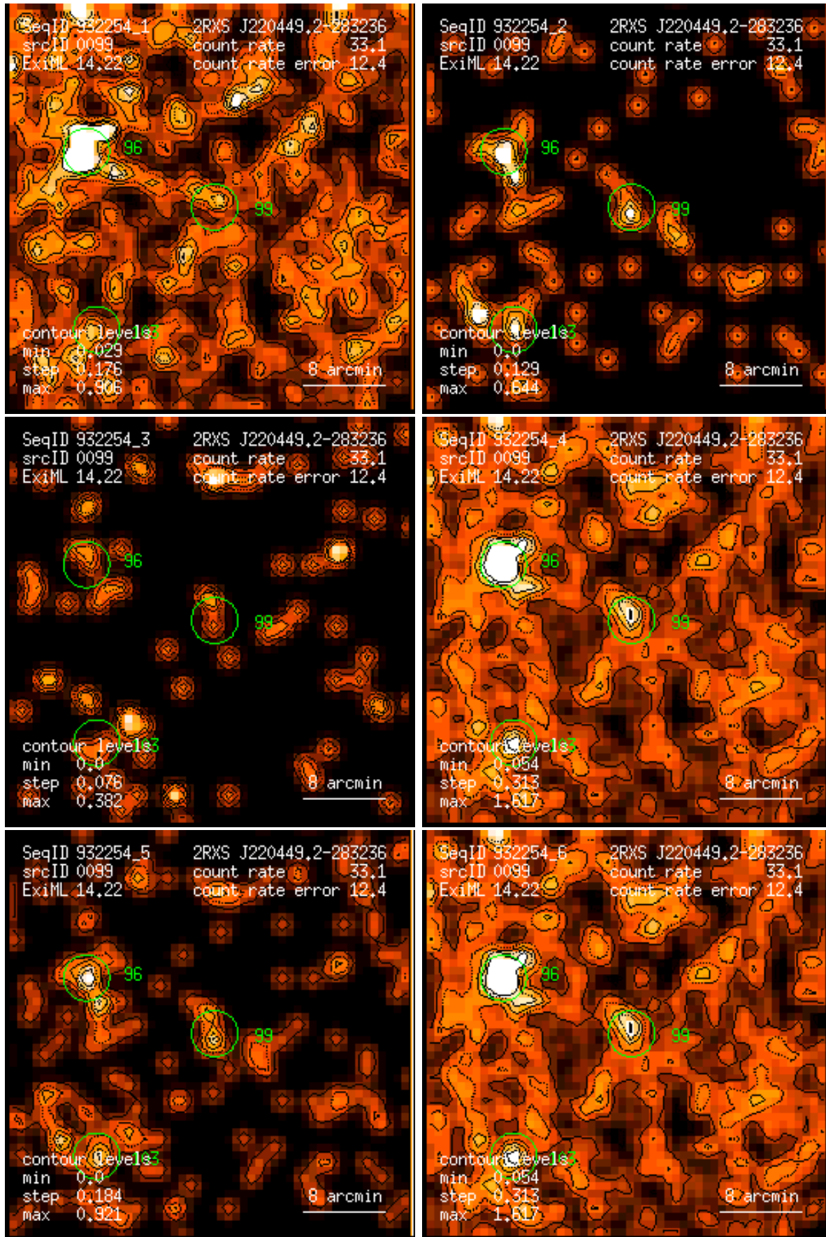
Figure 99: RASS 932254: detection 0099: band rate images, Gaussian filter: (1) PSPC channels 11 – 41, (2) 52 – 90, (3) 91 – 201, (4) 11 – 235, (5) 52 – 201, (6) 11 – 201. Broad band rates in counts/ks. Band rate contour levels in counts/ks/arcmin 2 .
