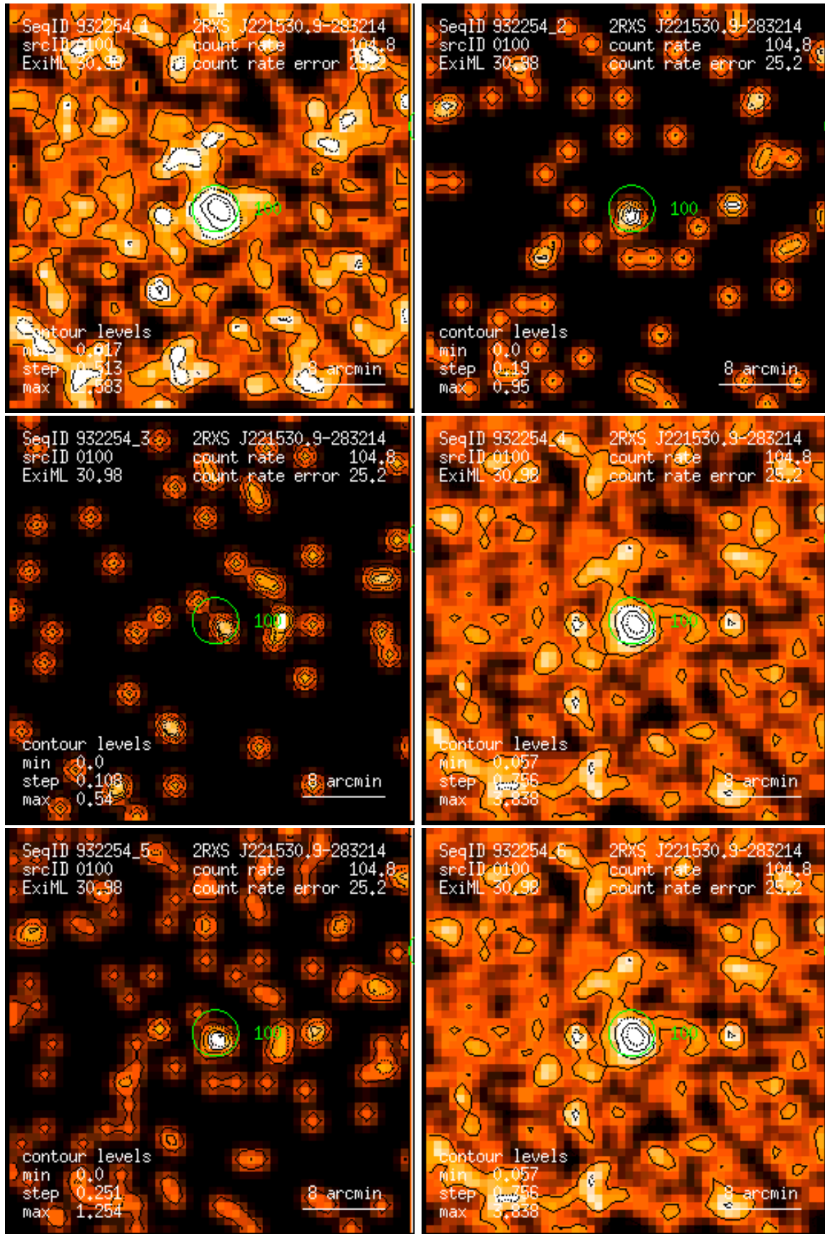
Figure 100: RASS 932254: detection 0100: band rate images, Gaussian filter: (1) PSPC channels 11 – 41, (2) 52 – 90, (3) 91 – 201, (4) 11 – 235, (5) 52 – 201, (6) 11 – 201. Broad band rates in counts/ks. Band rate contour levels in counts/ks/arcmin 2 .
