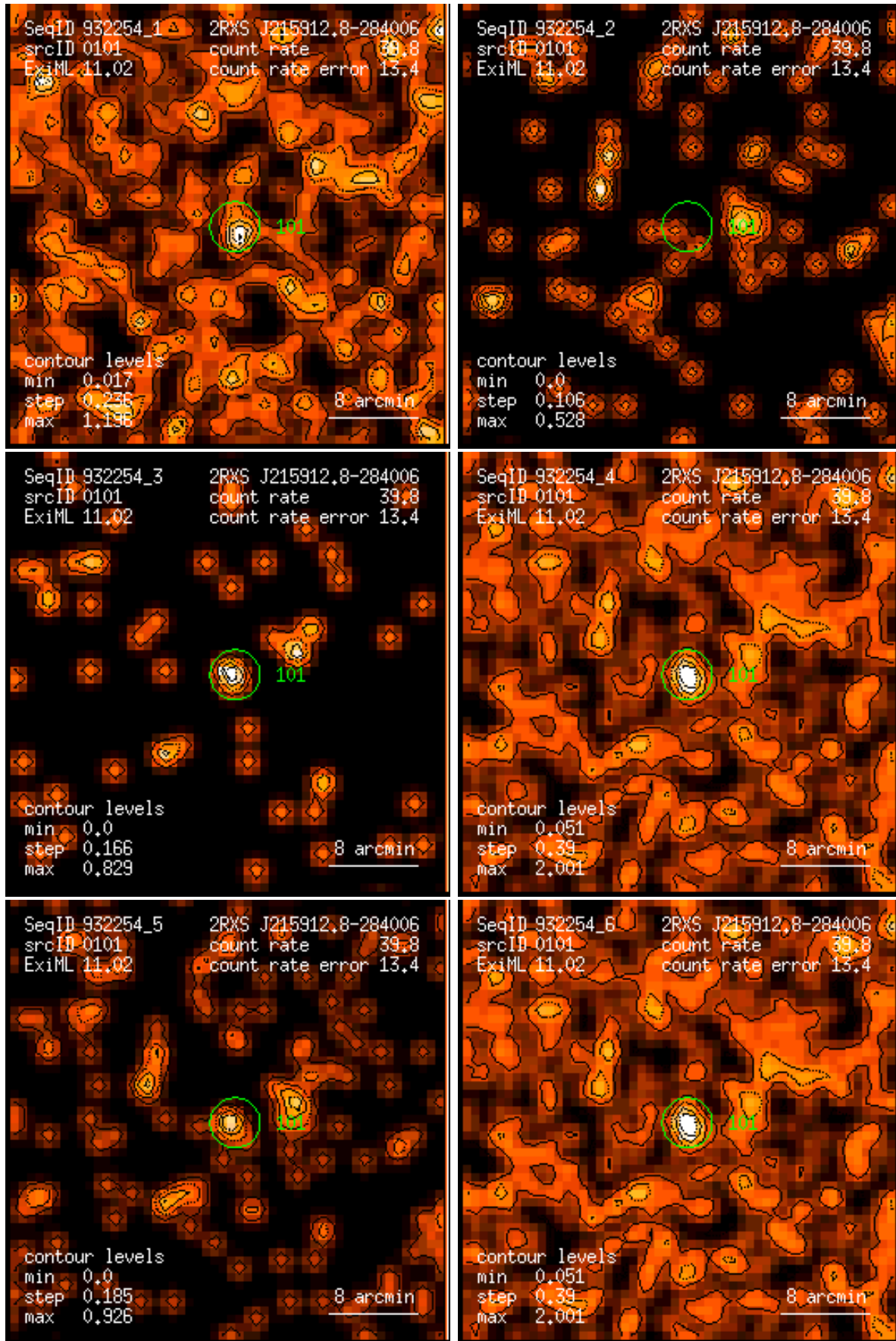
Figure 101: RASS 932254: detection 0101: band rate images, Gaussian filter: (1) PSPC channels 11 – 41, (2) 52 – 90, (3) 91 – 201, (4) 11 – 235, (5) 52 – 201, (6) 11 – 201. Broad band rates in counts/ks. Band rate contour levels in counts/ks/arcmin 2 .
